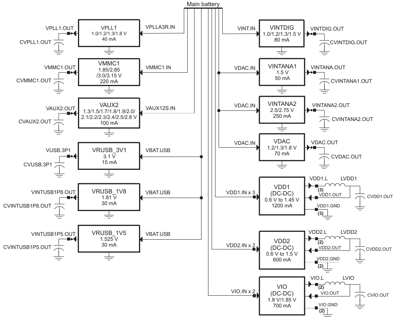
Figure 5-1. Power Provider Block Diagram
