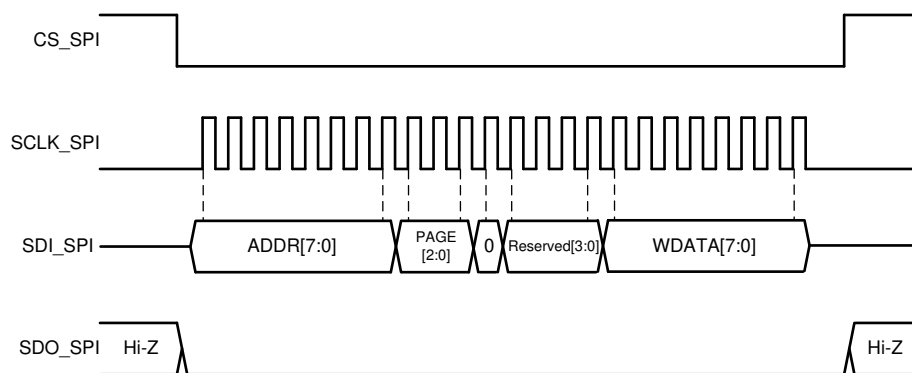
图 8-58. SPI Write Cycle
