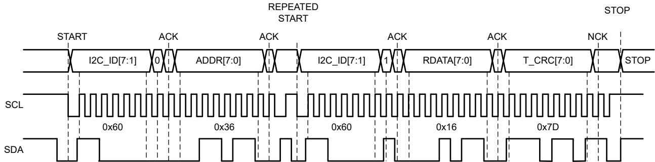
图 8-57. I²C READ Cycle with CRC
