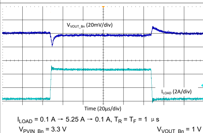
图 9-43. Buck Load Step Transient - 3-Phase, 4.4 MHz, Auto Mode
