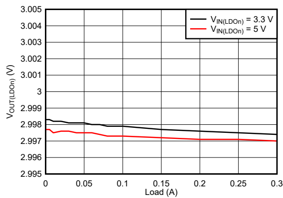
图 9-66. LDO4 Load Regulation, V_{out} = 3\text{ V}
