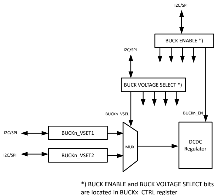
图 8-5. AVS/DVS Configuration Register Arbitration Diagram
