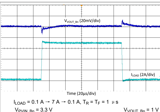
图 9-41. Buck Load Step Transient - 4-Phase, 4.4 MHz, Forced-PWM Mode
