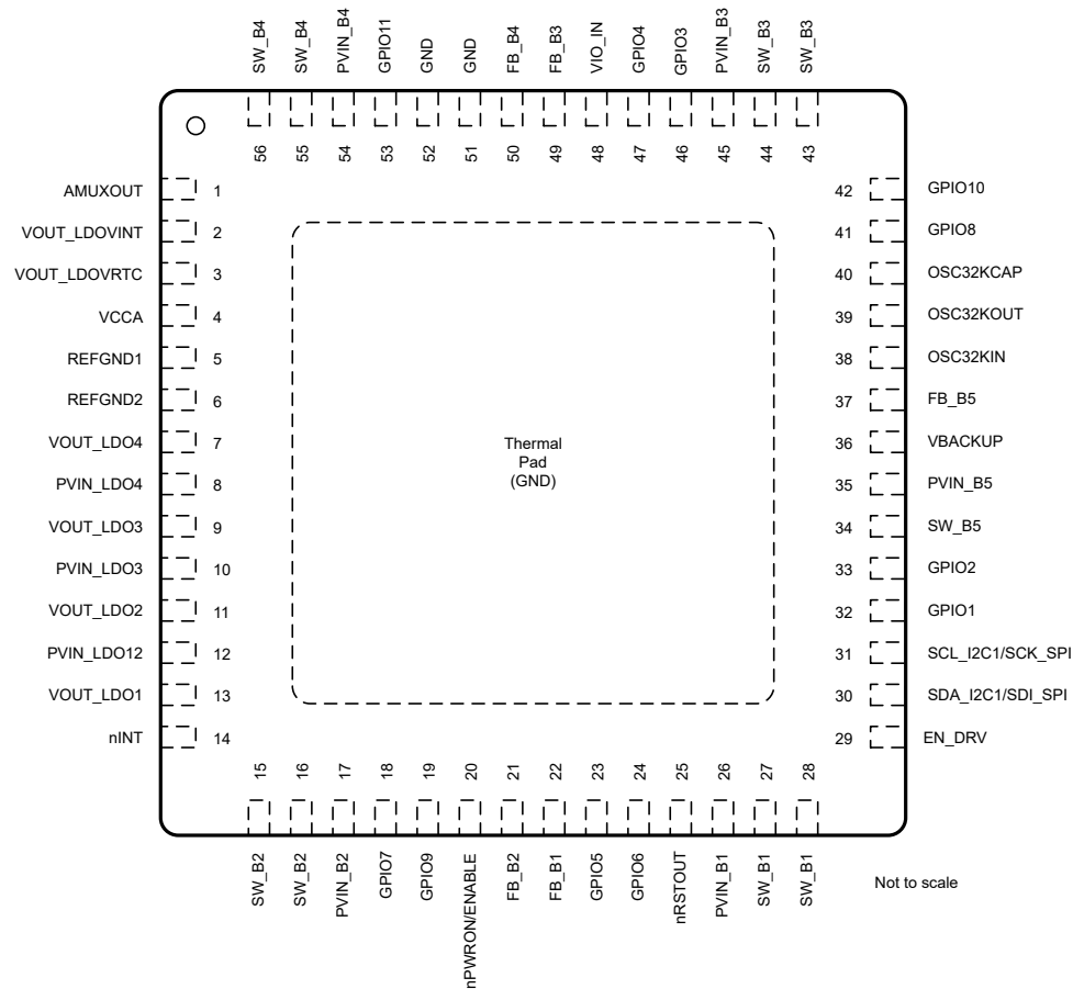
图 6-1. 56-Pin RWE (VQFNP) Package, 0.5-mm Pitch, With Thermal Pad (Top View)
