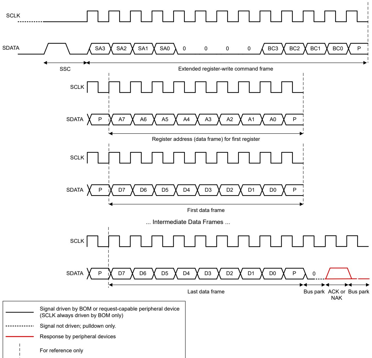
图 8-46. SPMI Extended Register Write Command
