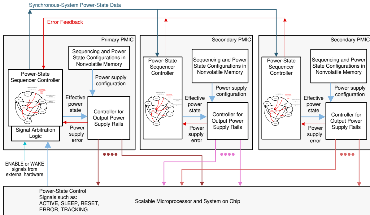
图 8-43. Multi-PMIC Power State Synchronization Block Diagram
