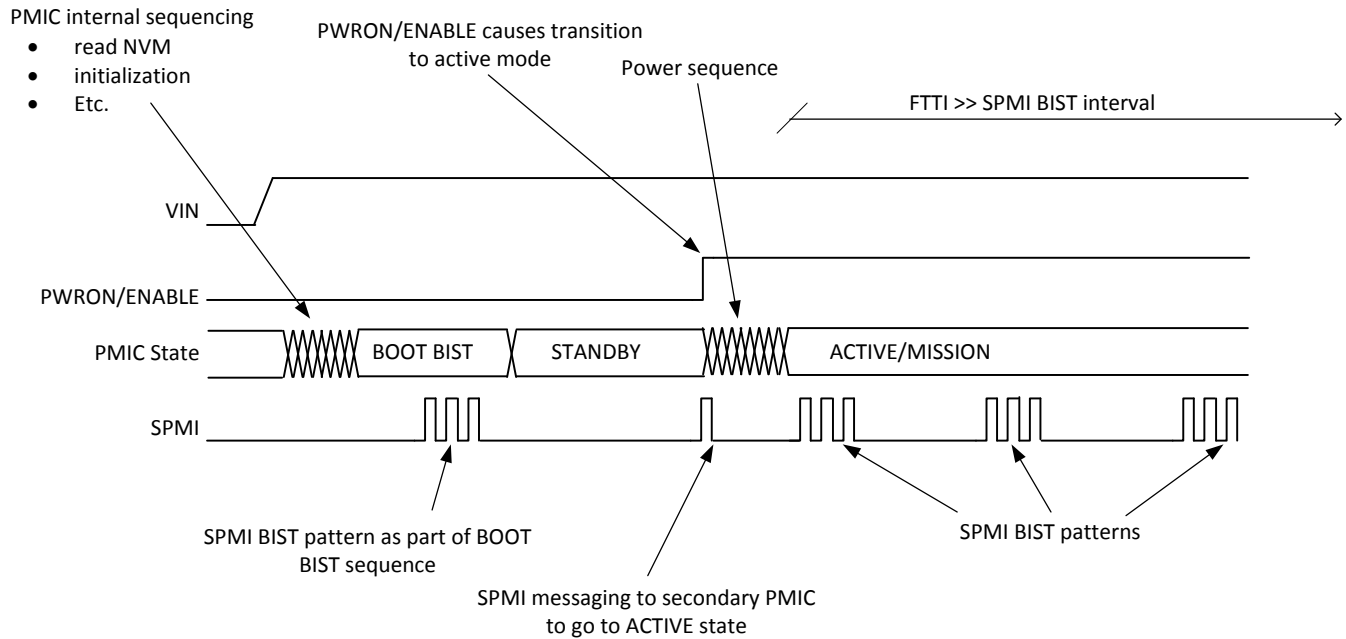
图 8-47. SPMI-BIST Operation
