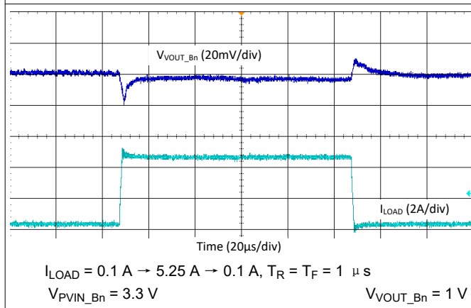
图 9-42. Buck Load Step Transient - 3-Phase, 2.2 MHz, Auto Mode
