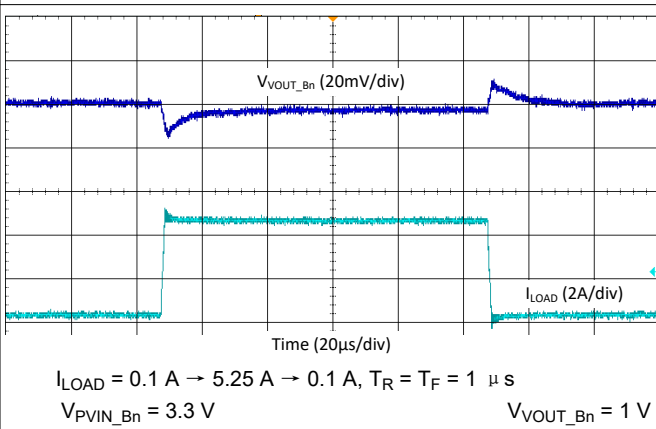
图 9-45. Buck Load Step Transient - 3-Phase, 4.4 MHz, Forced-PWM Mode
