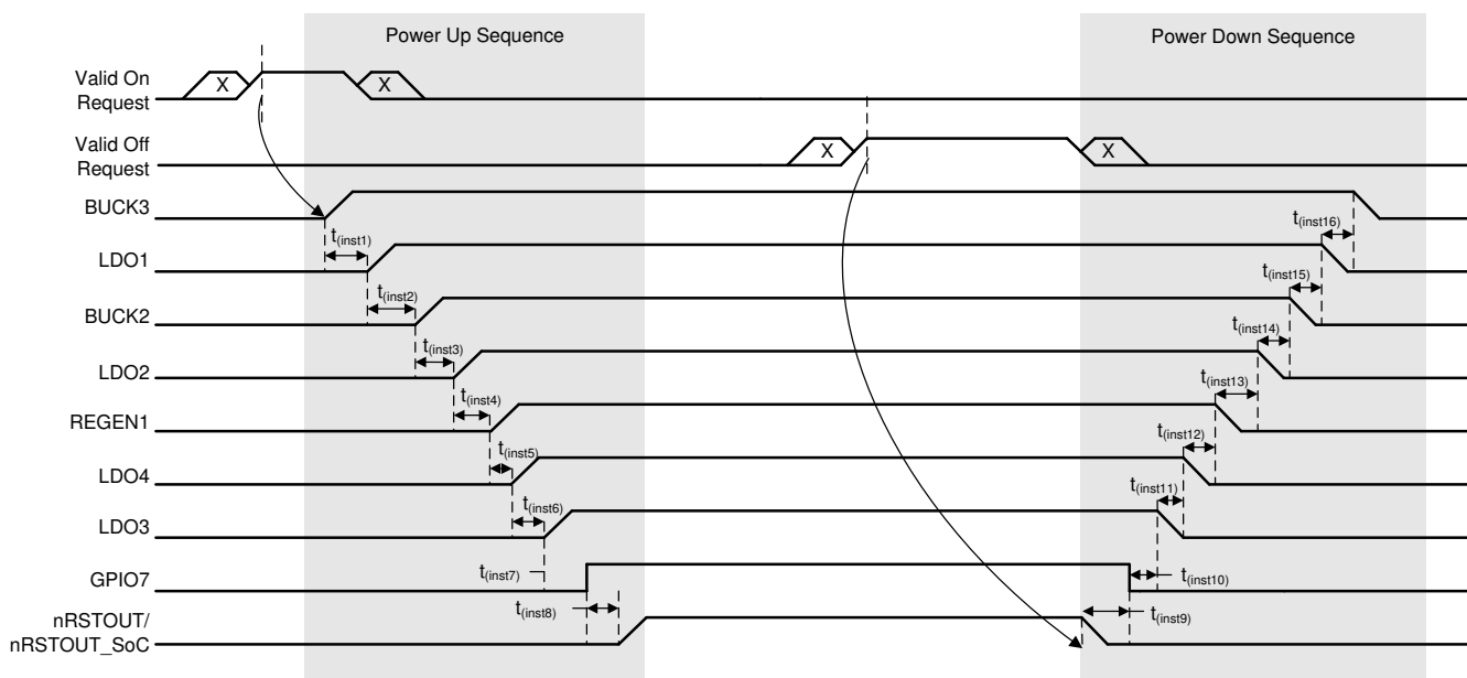
图 8-42. Power Sequence Example
