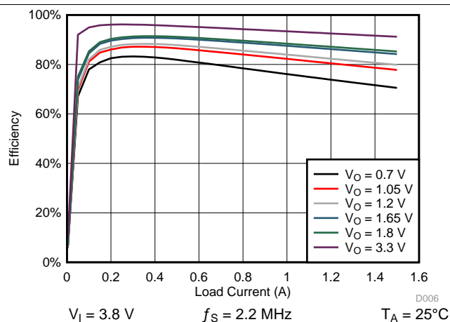
图 4-9. SMPS Efficiency for SMPS4 in PWM Mode
