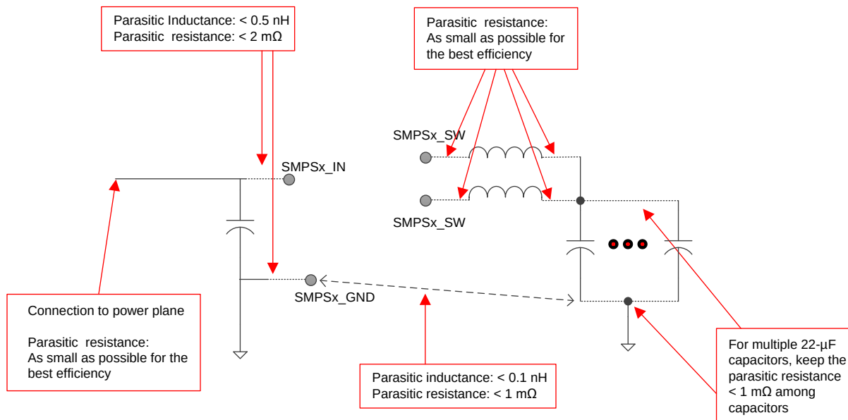
图 6-9. Parasitic Inductance and Resistance
