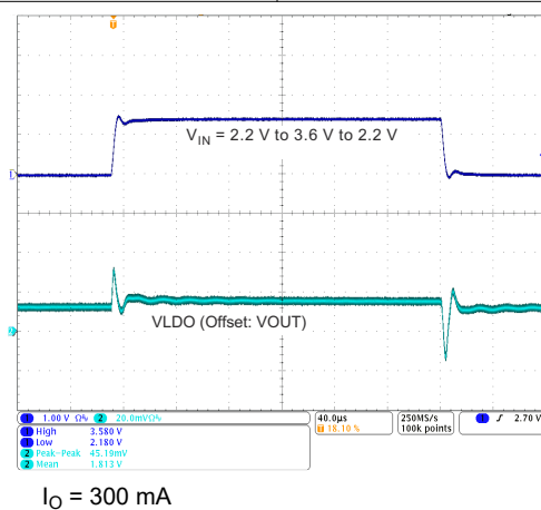
图 9-24. LDO10 Line Transient Response
