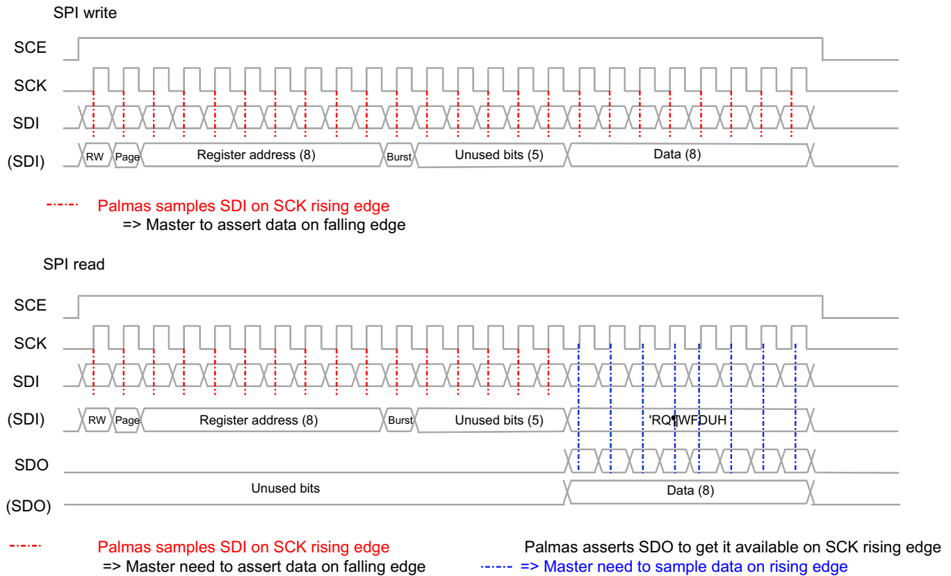
图 6-15. SPI Single Read and Write Access
