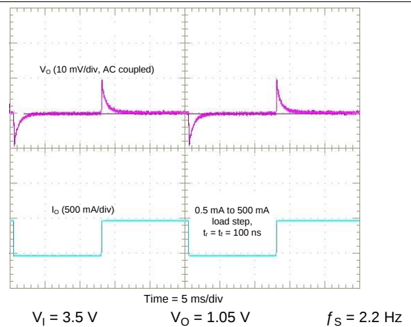
图 7-14. Typical SMPS Load Transient Response for SMPS12, SMPS3, SMPS45, SMPS6 and SMPS7
