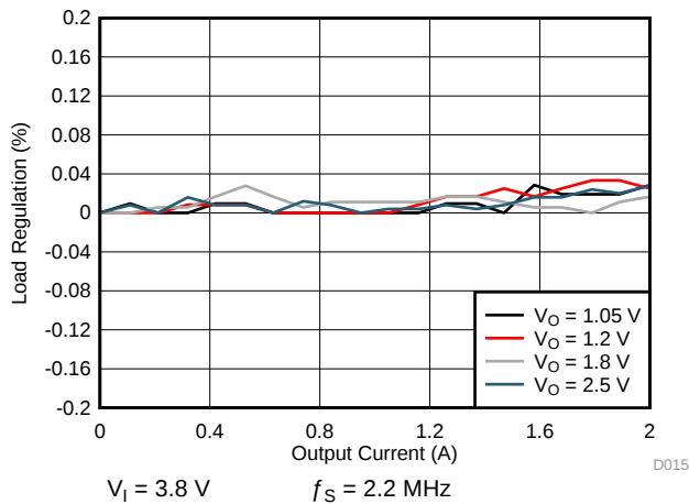
图 7-11. SMPS Regulation for 2-A Single Phase
