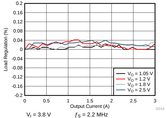
图 7-10. SMPS Load Regulation for 3-A Single Phase
