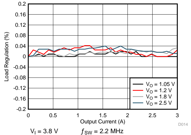
图 6-10. SMPS Load Regulation for 3-A Single Phase
