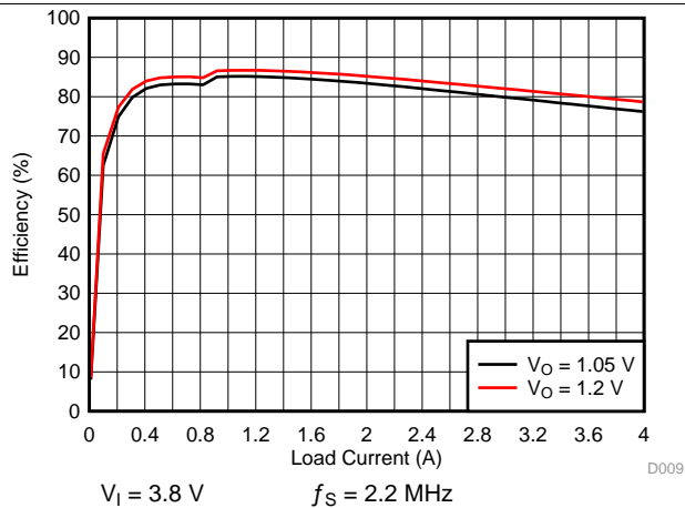
图 4-5. SMPS Efficiency for 4-A Multi-Phase PWM Mode
