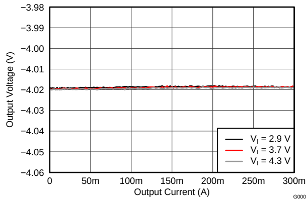
Figure 15. V_{NEG} Load Regulation
