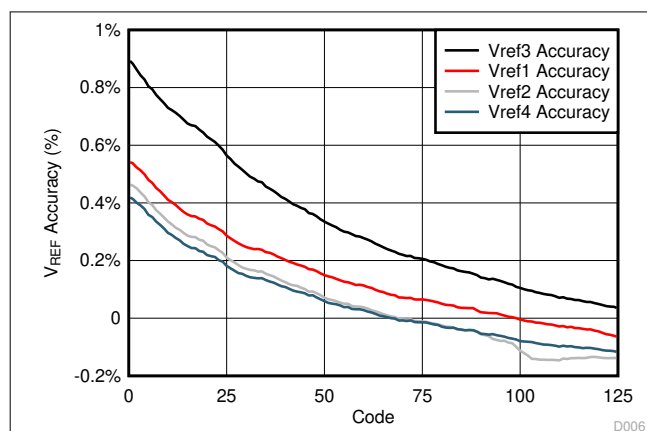
图 9-5. V_{REF} Accuracy vs Code
