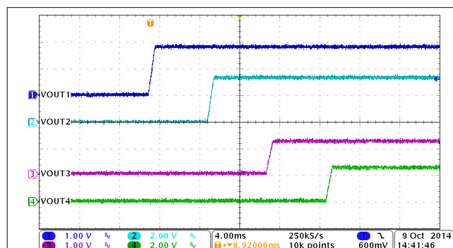
图 9-3. Configurable Power-Up Sequence
