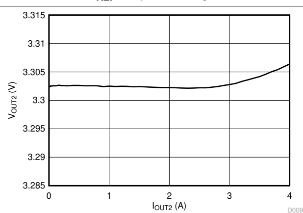
图 9-8. V_{OUT2} Load Regulation
