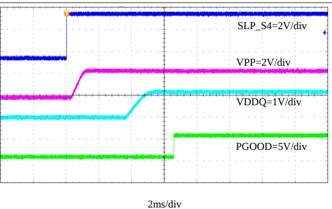
图 45. Start-Up Through SLP_S4, I_{VPPOUT} = 1\text{ A} , I_{VDQOUT} = 8\text{ A}
