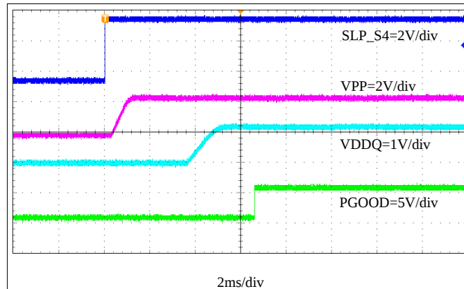
图 44. Start-Up Through SLP_S4, I_{VPPOUT} = 0\text{ A} , I_{VDQOUT} = 0\text{ A}
