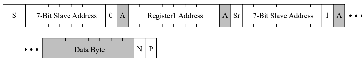
Figure 39. I 2 C Read Data Format
