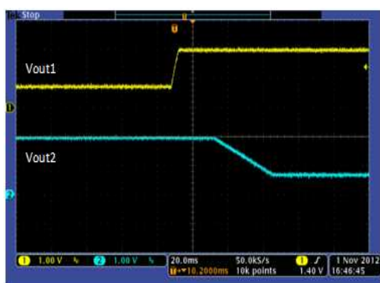
Figure 30. Voltage Change With I 2 C Control Buck 1, 0.68 V - 1.95 V, SR = 10\text{ mV}/16\text{ Tsw} , Buck 2, 1.95 V - 0.68 V, SR = 10\text{ mV}/128\text{ Tsw}
