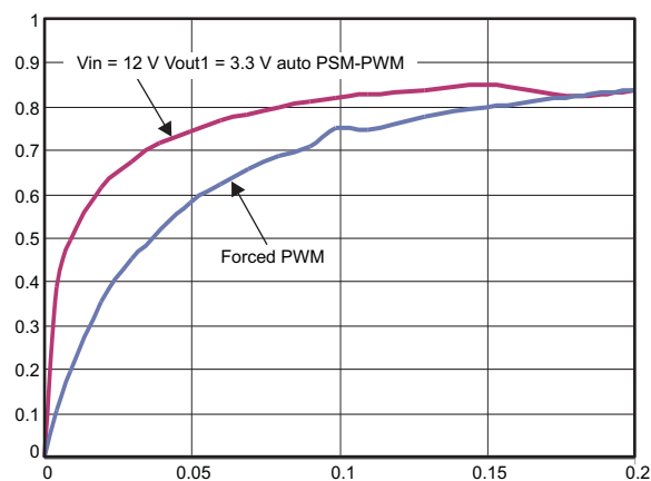
Figure 5. Efficiency Buck 1 at 3.3 V
