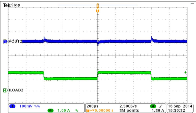
Figure 43. Buck2, Load Transient, 1.0 to 1.5 A
