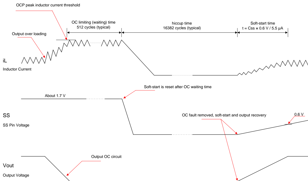
Figure 29. Overcurrent Protection
