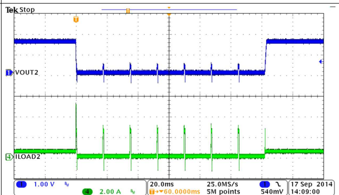
Figure 45. Buck3, Load Transient, 1.0 to 1.5 A
