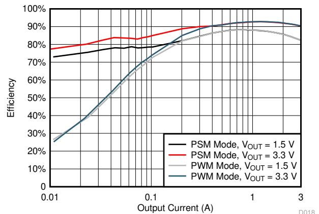
图 7-18. Buck2 Efficiency, V_{IN} = 12\text{ V} , F_{sw} = 610\text{ kHz}
