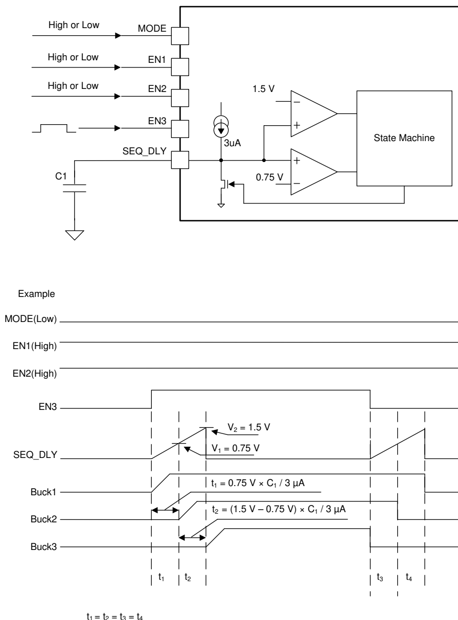
图 8-6. Automatic Power Sequencing
