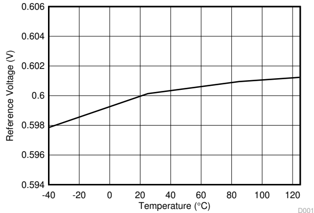
图 7-1. Voltage Reference vs Temperature
