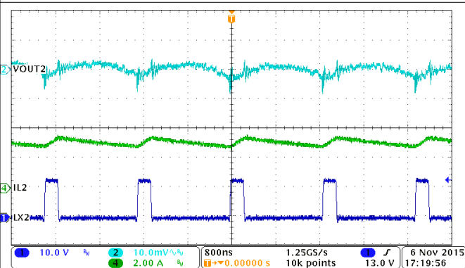
图 9-20. Buck2, Output Ripple, Iout = 3 A
