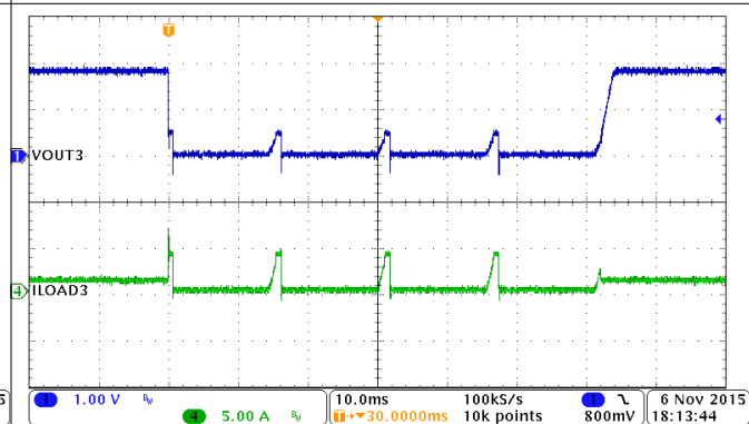
图 9-32. Buck3, Hiccup and Recovery
