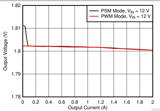
图 7-22. Buck3, Load Regulation
