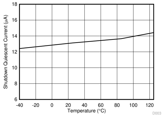
图 7-3. Shutdown Quiescent vs Temperature
