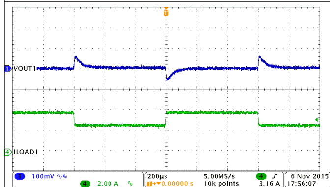
图 9-25. Buck1, Load Transient, 2.5 A to 3.75 A, SR 0.25 A/μs
