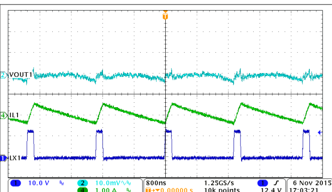
图 9-16. Buck1, FCC Mode, Iout = 0 A
