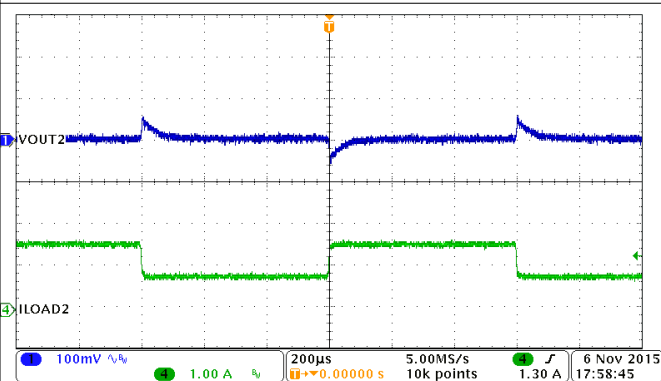
图 9-26. Buck2, Load Transient, 0.75 A to 1.5 A, SR 0.25 A/μs
