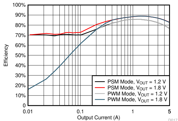
图 7-17. Buck1 Efficiency, V_{IN} = 12\text{ V} , F_{sw} = 610\text{ kHz}
