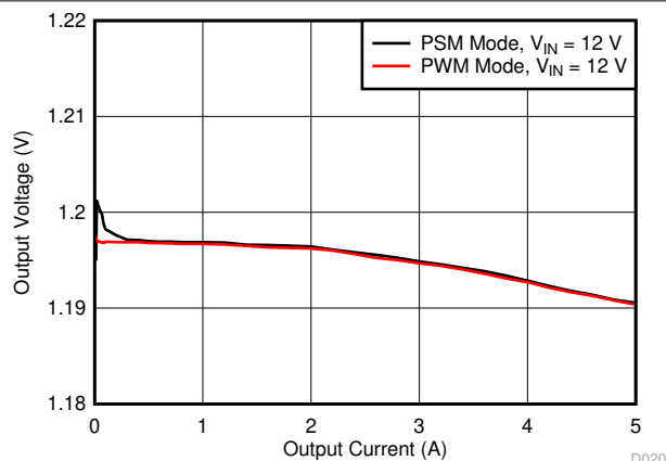
图 7-20. Buck1, Load Regulation
