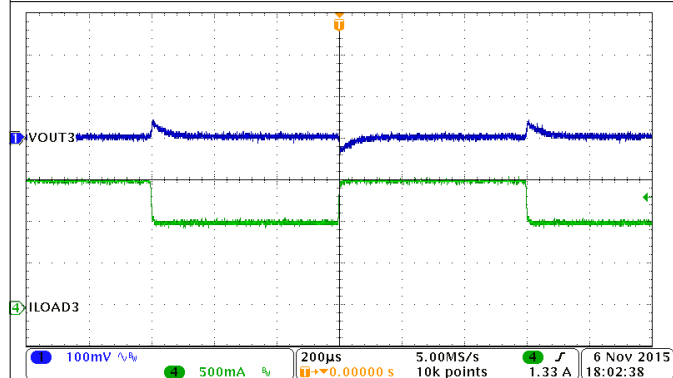
图 9-29. Buck3, Load Transient, 1 A to 1.5 A, SR 0.25 A/µs
