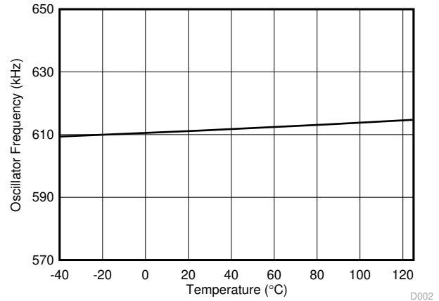
图 7-2. Oscillator Frequency vs Temperature
