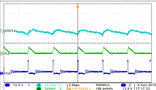
图 9-18. Buck2, PSM Mode, Output Ripple, Light Load
