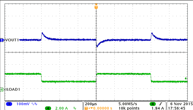
图 9-24. Buck1, Load Transient, 1.25 A to 2.5 A, SR 0.25 A/μs
