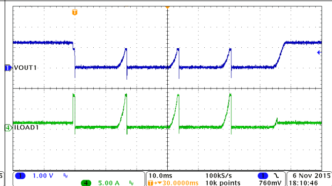
图 9-30. Buck1, Hiccup and Recovery
