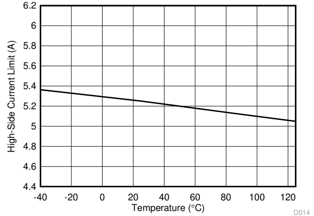
图 7-14. Buck2 High-Side Current Limit vs Temperature
