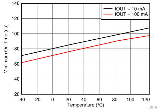
图 7-16. Minimum On Time vs Temperature
