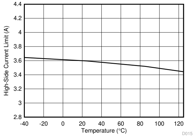
图 7-15. Buck3 High-Side Current Limit vs Temperature
