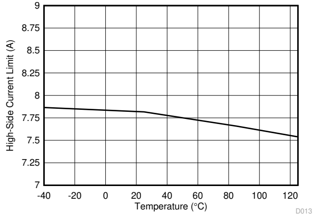
图 7-13. Buck1 High-Side Current Limit vs Temperature
