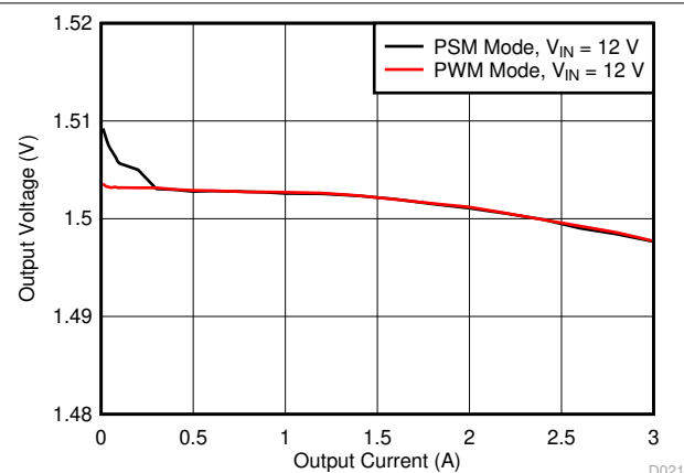
图 7-21. Buck2, Load Regulation
