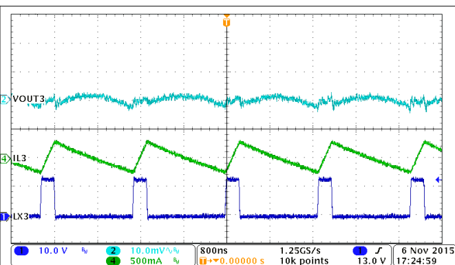
图 9-22. Buck3, FCC Mode, Iout = 0 A
