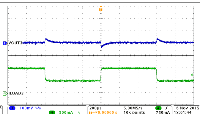
图 9-28. Buck3, Load Transient, 0.5 A to 1 A, SR 0.25 A/µs
