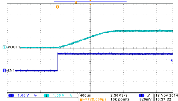
Iout = 3 A 图 8-3. BUCK1, Soft Start
