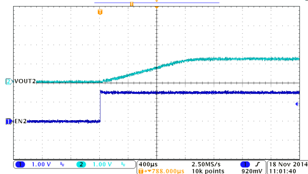
Iout = 2 A 图 8-4. BUCK2, Soft Start
