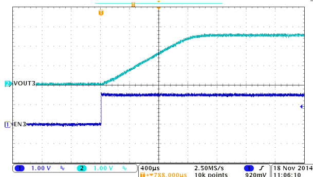
Iout = 2 A 图 8-5. BUCK3, Soft Start
