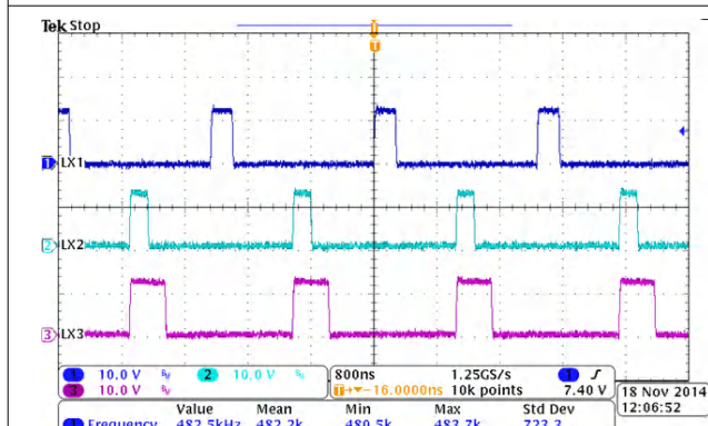
图 8-21. 180° Out-of-Phase
