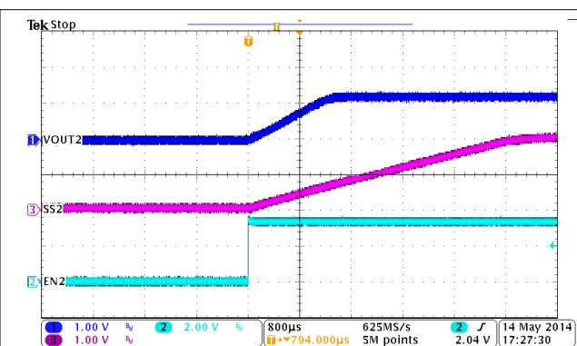
图 9-3. BUCK2, Soft-Start, Iout = 2 A
