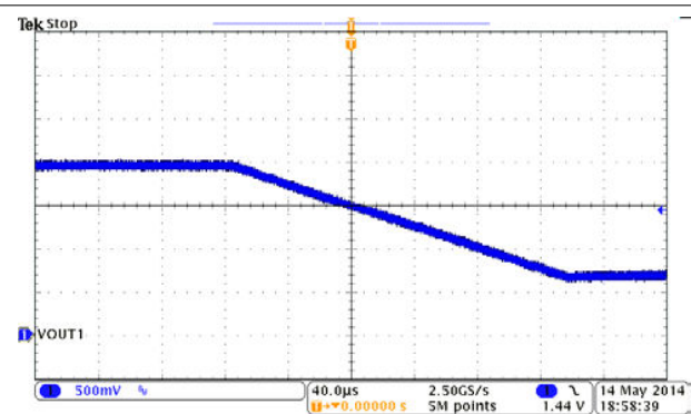
图 9-19. VID1 from 7F to 00, SR = 10 mV/cycle
