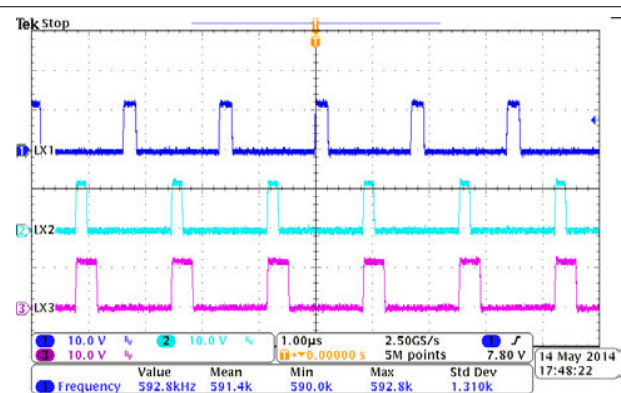
图 9-17. 180° Out-of-Phase
