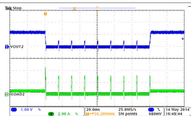
图 9-15. BUCK2, Hiccup and Recovery
