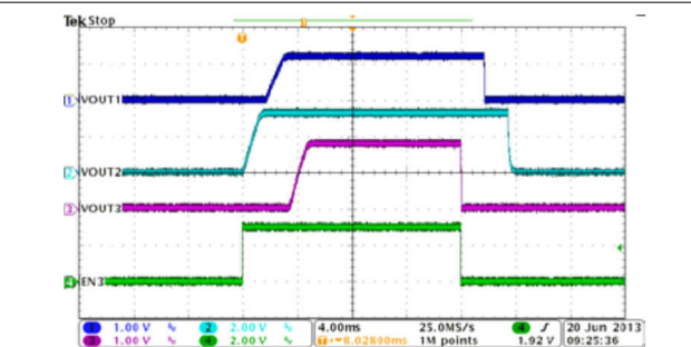
图 8-31. Automatic Power Sequencing, MODE=EN2=HIGH, EN1=LOW
