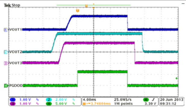
图 8-30. Automatic Power Sequencing, MODE=EN1=HIGH, EN2=LOW
