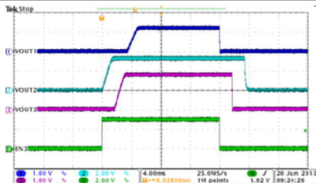
图 8-29. Automatic Power Sequencing, MODE=EN1= HIGH, EN2=LOW
