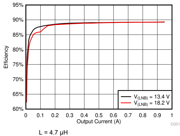
图 6-1. Power Efficiency
