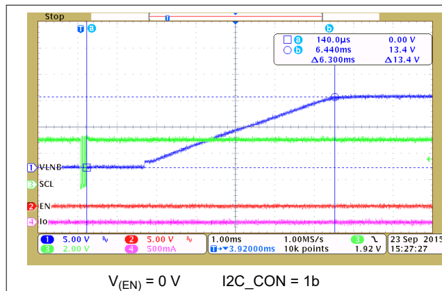
图 7-3. VLNB Output Controlled by bit EN of Control Register 2
