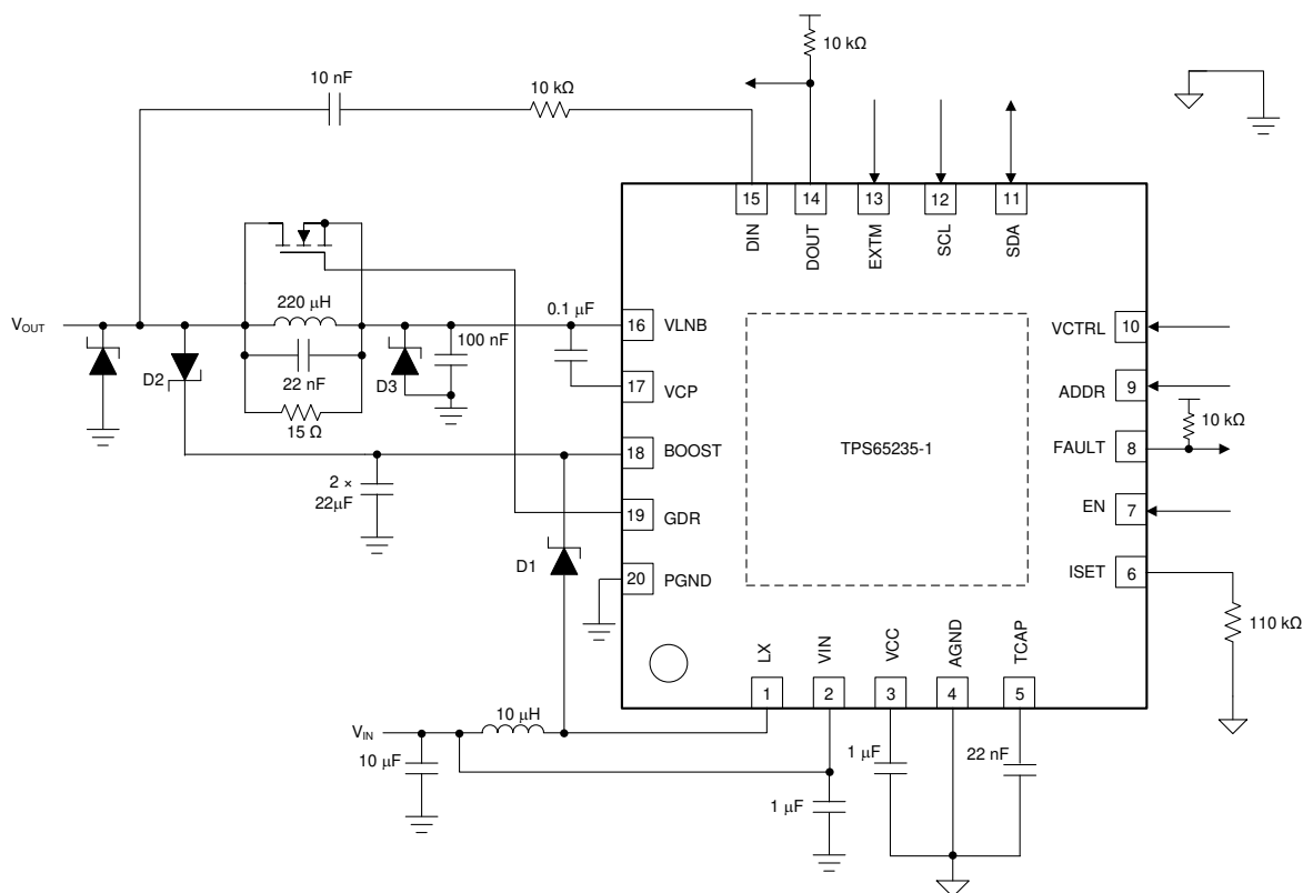
图 8-18. Application Schematic for DiSEqC2.x Support
