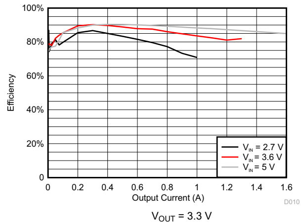
图 8-7. DCDC4 Efficiency
