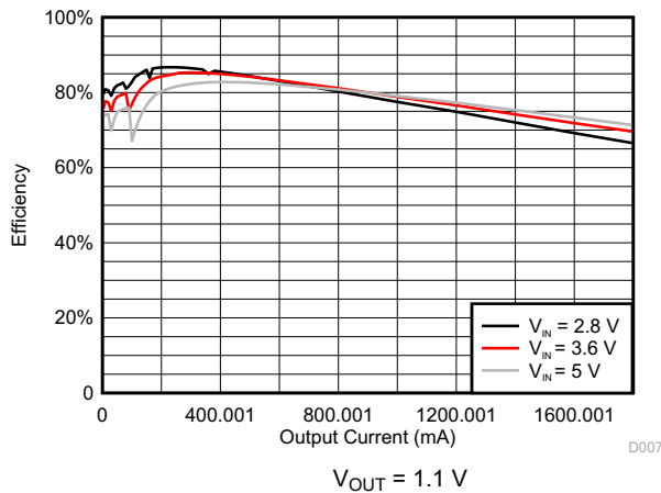
图 8-4. DCDC1/DCDC2 Efficiency
