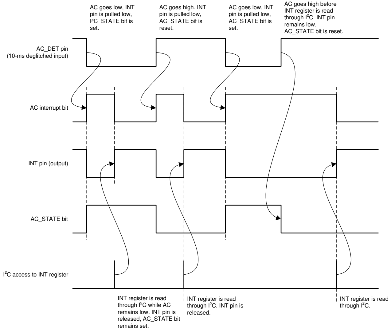
图 7-30. AC_STATE Pin
