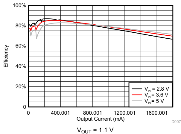
图 9-4. DCDC1/DCDC2 Efficiency
