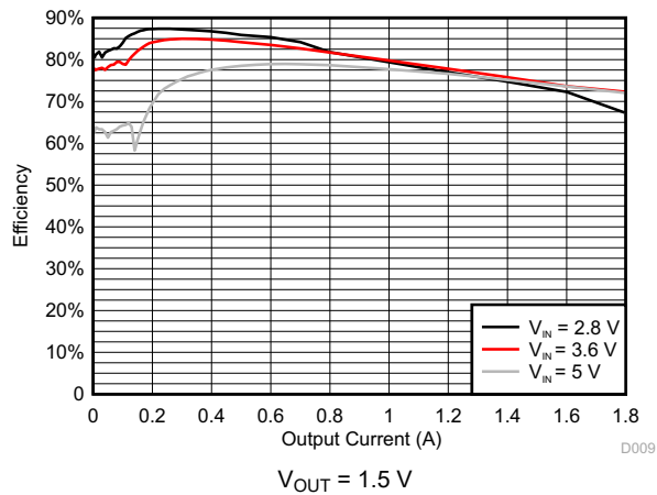
图 9-6. DCDC3 Efficiency
