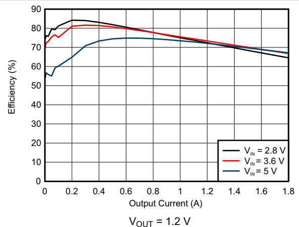
图 9-5. DCDC3 Efficiency
