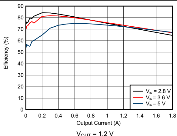
图 8-5. DCDC3 Efficiency
