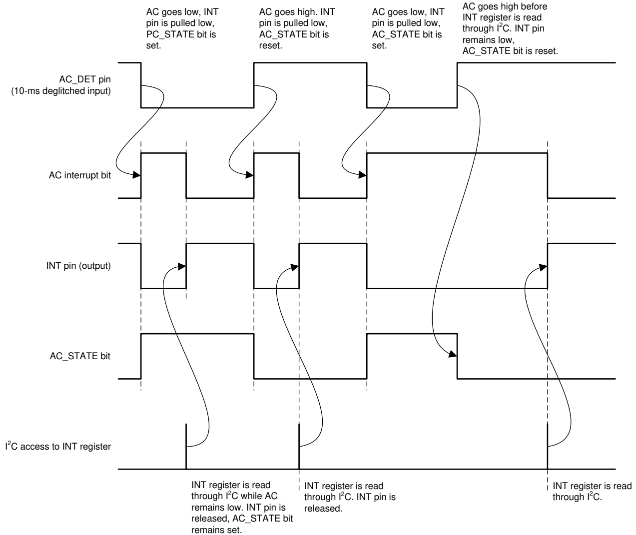
图 7-29. AC_STATE Pin
