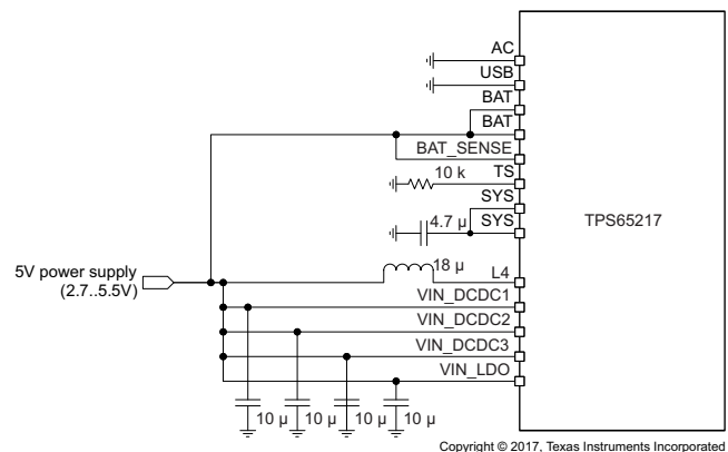
图 62. Power Connection for 5-V Only Operation Directly Wired to BAT Instead of a Battery
