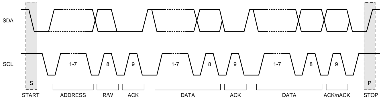
Figure 4-22. I²C Protocol and Transmission Timing; I²C Start/Stop/Acknowledge Protocol
