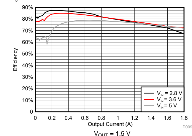
Figure 5-4. DCDC3 Efficiency
