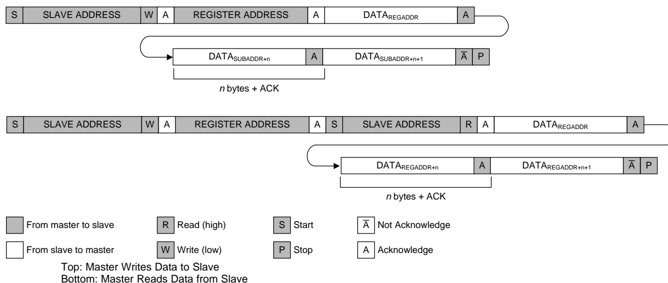
Figure 4-21. I 2 C Data Protocol
