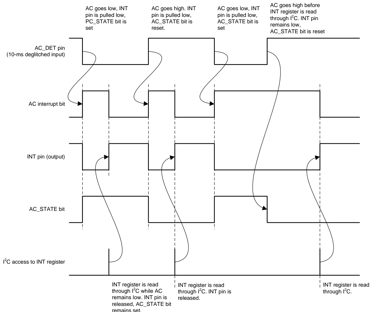
Figure 4-19. AC_STATE Pin
