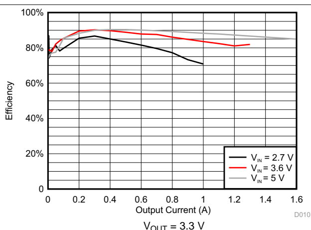
Figure 5-5. DCDC4 Efficiency
