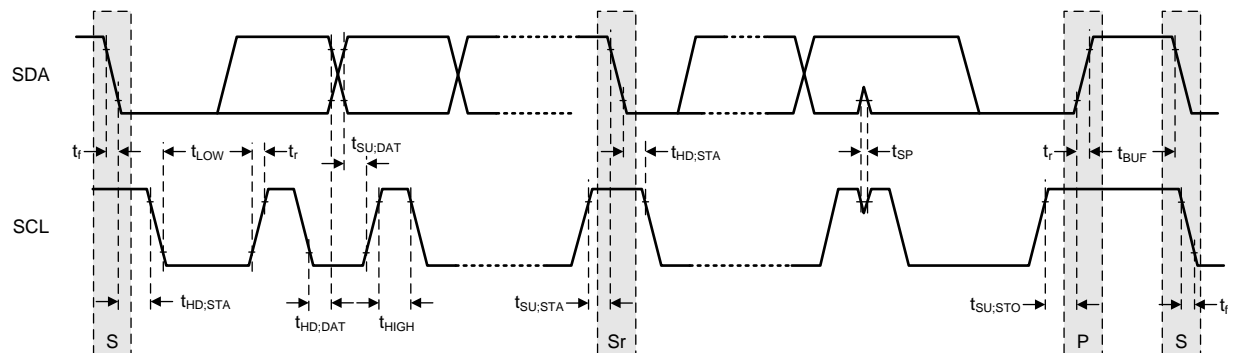
Figure 4-23. I²C Protocol and Transmission Timing; I²C Data Transmission Timing
