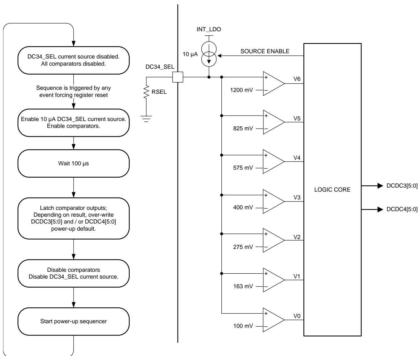
Figure 4-13. Left: Flow Chart for Selecting DCDC Power-Up Default Voltage Right: Comparator Circuit
