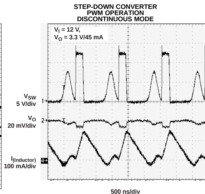
500 ns/div Figure 10.
