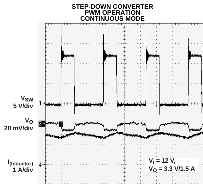
500 ns/div Figure 9.
