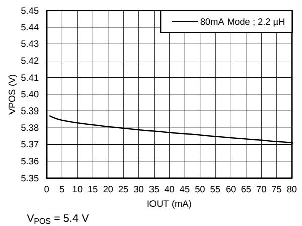
Figure 74. Load Regulation
