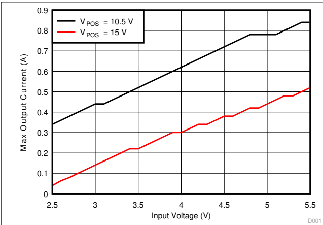
图 6-1. Boost Converter ( V_{\text{POS}} ) Maximum Output Current vs Input Voltage
