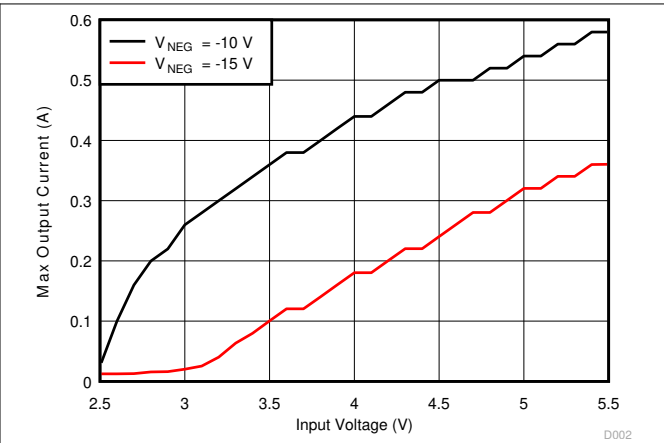
图 6-2. Inverting Converter ( V_{\text{POS}} ) Output Current vs Input Voltage
