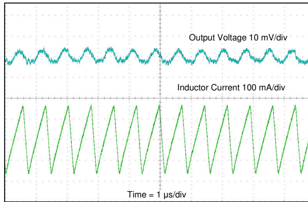
图 8-12. Inverting Converter ( V_{NEG} ) Output Ripple
