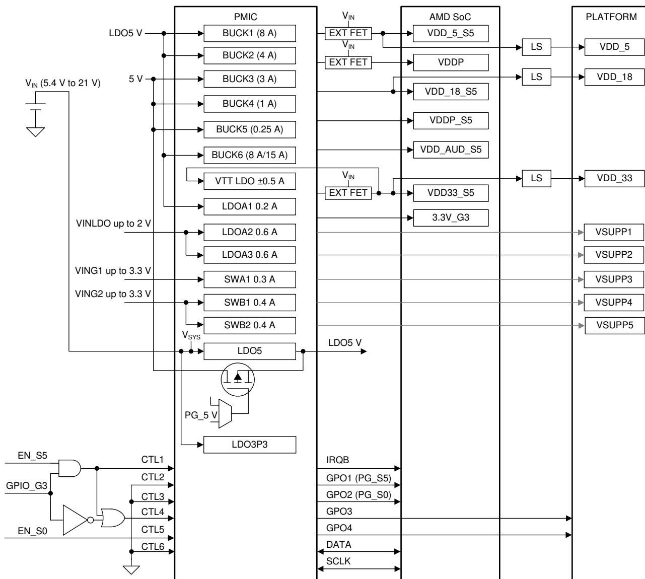
图 7-2. Typical Application Example
