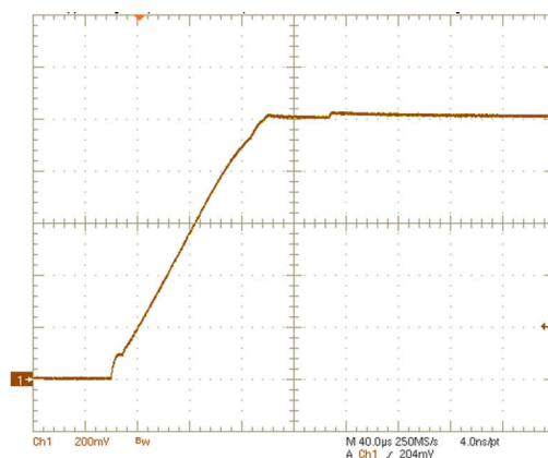
图 5-2. Converter Start Up to 1V by I²C
