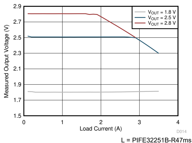
图 6-7. Converter Load Current Limitations with V_{IN} = 3.3\text{V}
