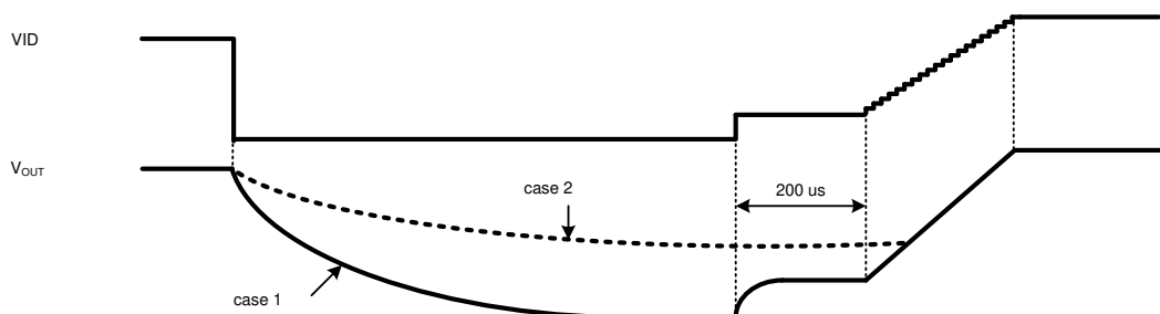
图 7-22. Decay Down to 0 V and Slew Up
