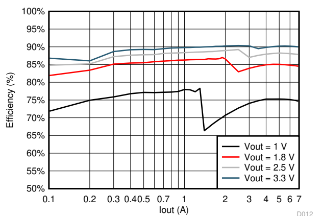
FET = CSD87381P L = PIMB061H-R47ms BUCK1_MODE = 0b
