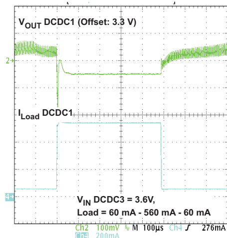
Figure 12. Load Transient Response Converter 1
