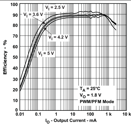
Figure 49. DCDC2 Efficiency
