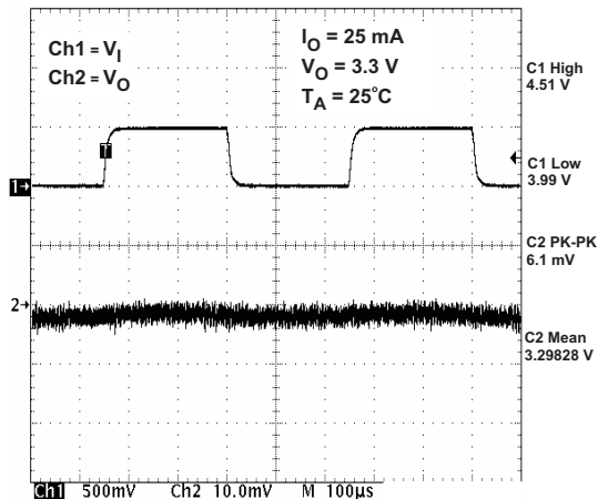
Figure 22. LDO2 Line Transient Response
