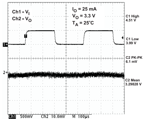
Figure 24. LDO2 Line Transient Response
