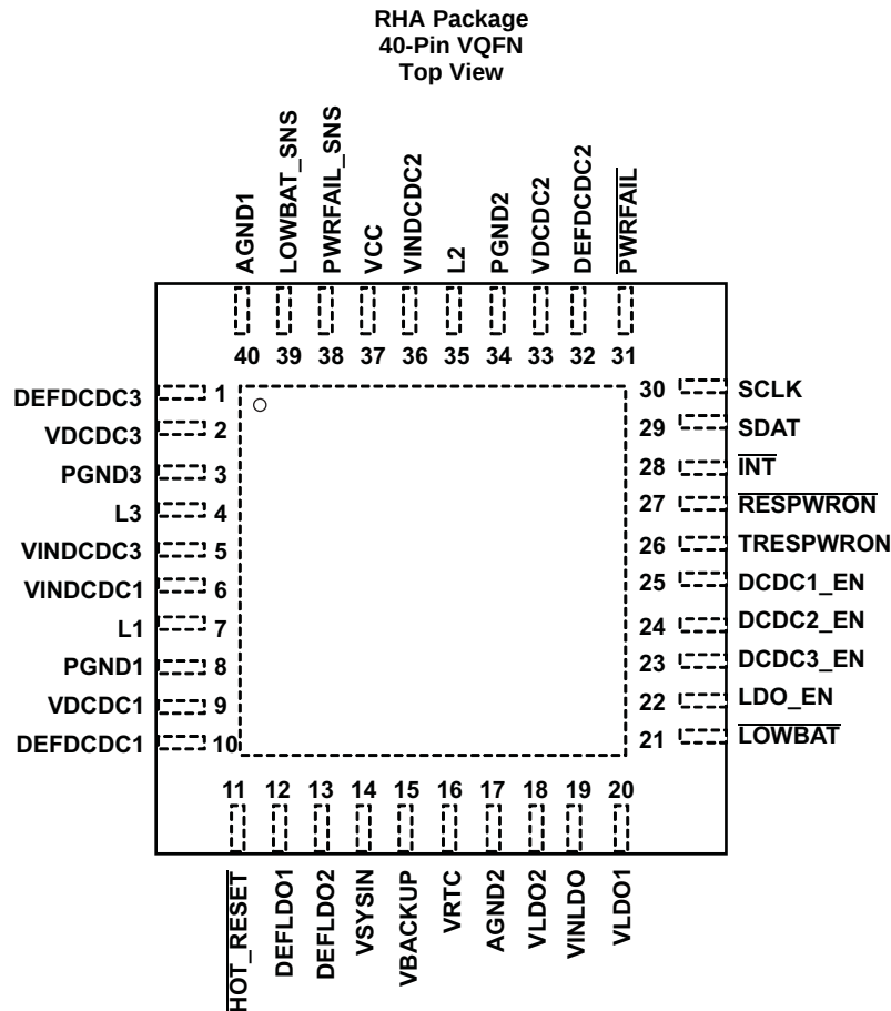
Pin Functions
