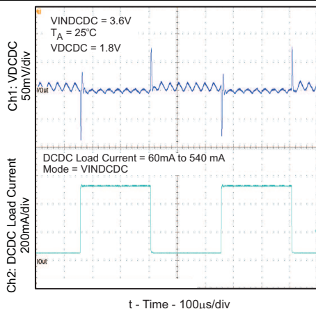
Figure 11. Load Transient Response (DC-DC PWM Mode)
