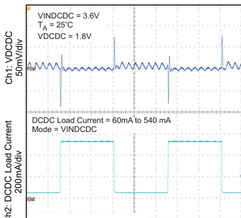
Figure 28. Load Transient Response (DC-DC PWM Mode)
