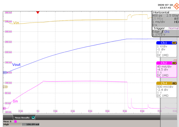
图 8-38. Start-up with 100-mA ICL
