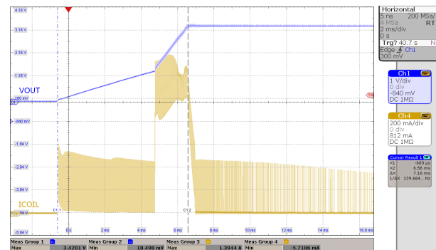
图 8-31. Start-up Behavior from Rising Enable
