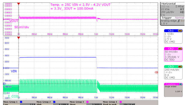
图 8-21. Line Transient, High Load
