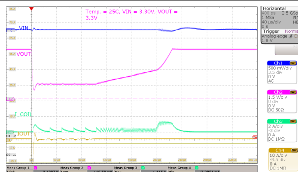
图 8-38. Start-up with 100-mA ICL
