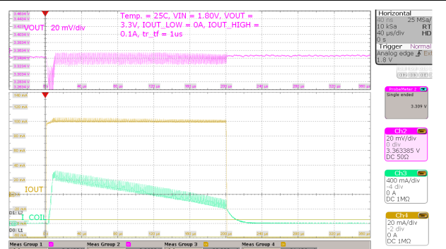
图 8-20. Line Transient, Light Load
