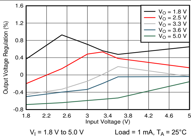
图 8-19. Line Regulation
