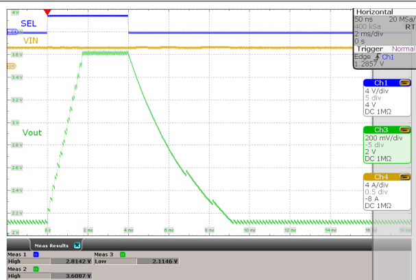
图 8-40. Short Circuit Behavior
