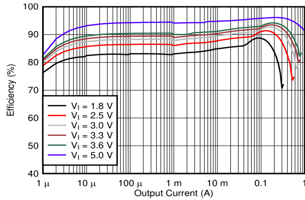
图 8-8. Efficiency versus Output Current
