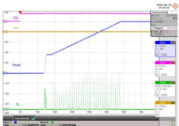
图 8-28. Start-up Behavior from Rising Enable
