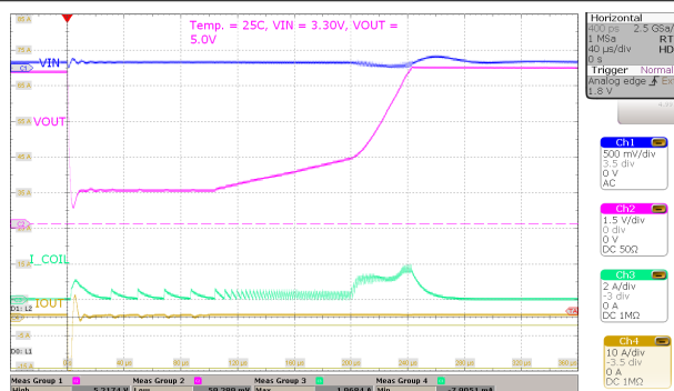
图 8-41. Short Circuit Behavior
