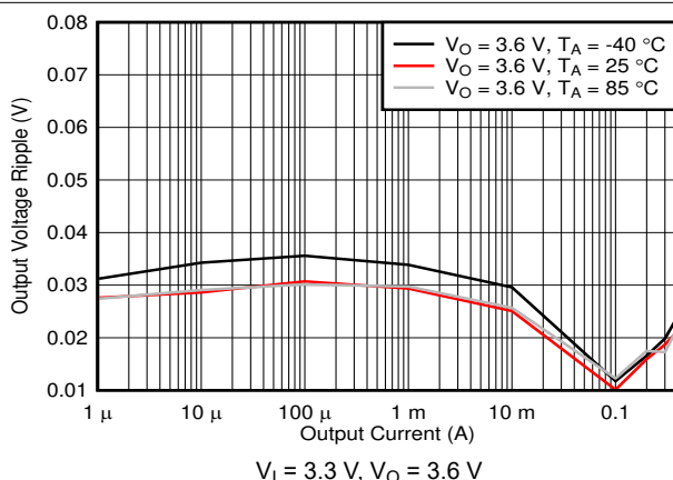
图 8-17. Output Voltage Ripple over Temperature
