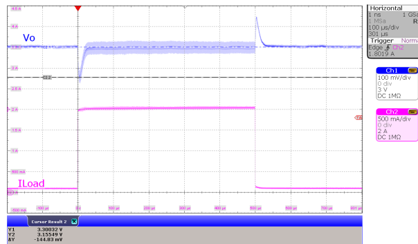
V_I = 2.8\text{ V} , V_O = 3.3\text{ V} I_O from 100 mA to 2 A t_r = 1\text{ }\mu\text{s} , t_f = 1\text{ }\mu\text{s} TPS63806 MODE = High
