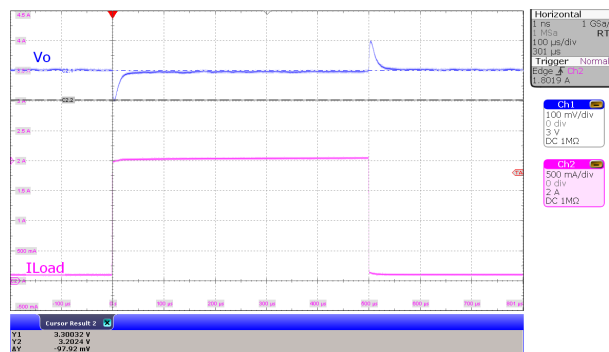
V_I = 4.2\text{ V} , V_O = 3.3\text{ V} I_O 100 mA to 2 A t_r = t_f = 1\text{ }\mu\text{s} TPS63806 MODE = High
