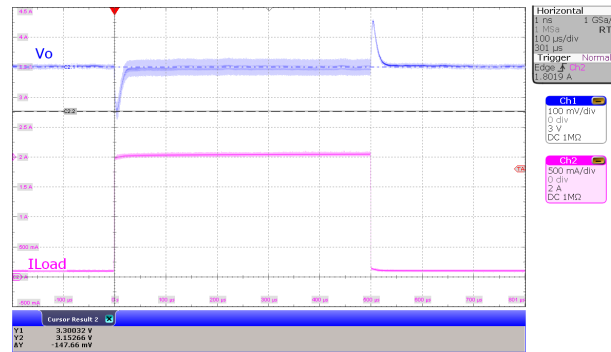
V_I = 3.3\text{ V} , V_O = 3.3\text{ V} I_O 100 mA to 2 A t_r = t_f = 1\text{ }\mu\text{s} TPS63806 MODE = High
