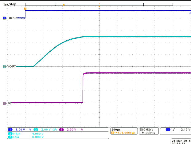
Figure 50. Start-up Timing
