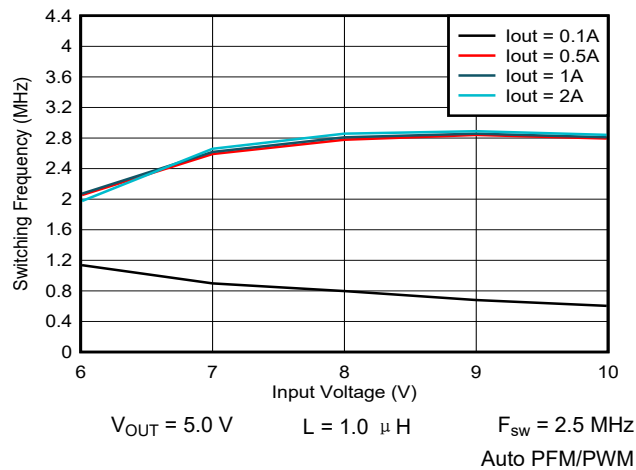
图 9-42. Switching Frequency vs Input Voltage
