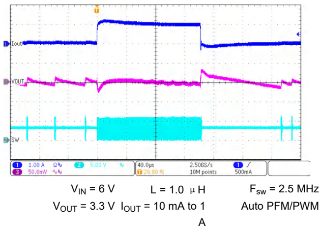
图 9-72. Load Transient Response
