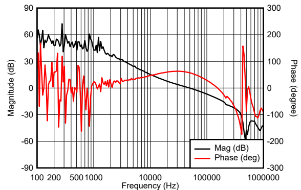
图 10-7. 环路频率响应, I_{OUT} = 3A , BW = 49.4kHz , PM = 57^\circ , GM = -12dB
