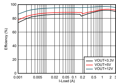
TPS62933 效率 (VIN = 24V, fSW = 500kHz)
