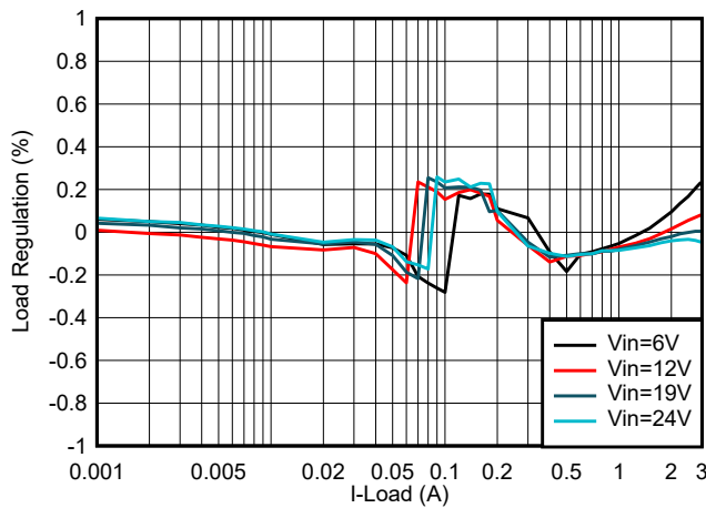
图 8-25. TPS62933 负载调节, V_{OUT} = 3.3\text{V} , f_{SW} = 1200\text{kHz}
