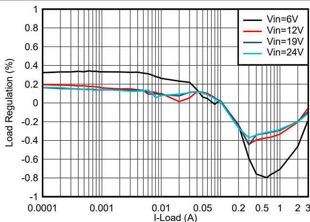
图 8-29. TPS62933O 负载调节, V_{OUT} = 5\text{V} , f_{SW} = 500\text{kHz}
