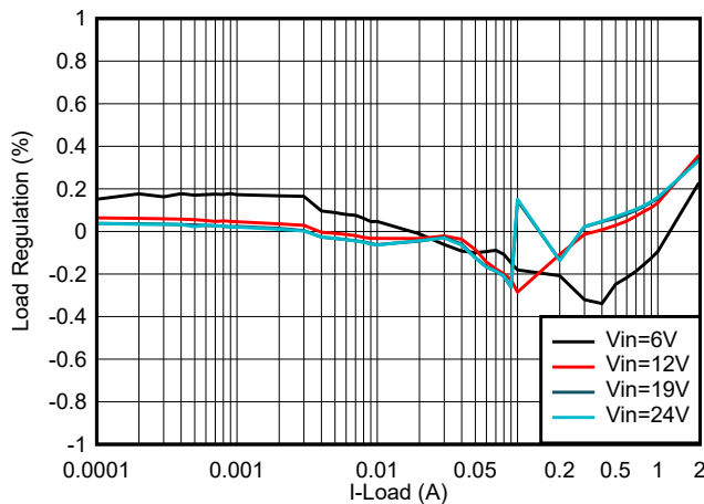
图 8-27. TPS62932 负载调节, V_{OUT} = 5\text{V} , f_{SW} = 500\text{kHz}
