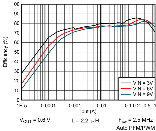
图 9-50. Efficiency vs Output Current
