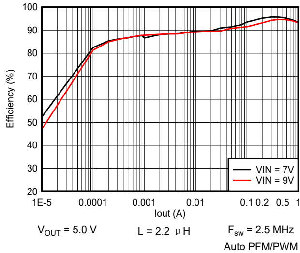
图 9-2. Efficiency vs Output Current
