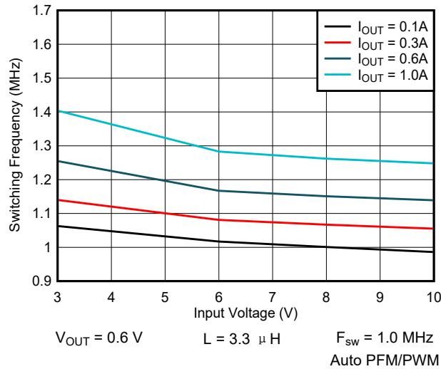
图 9-58. Switching Frequency vs Input Voltage
