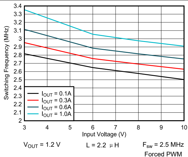
图 9-41. Switching Frequency vs Input Voltage
