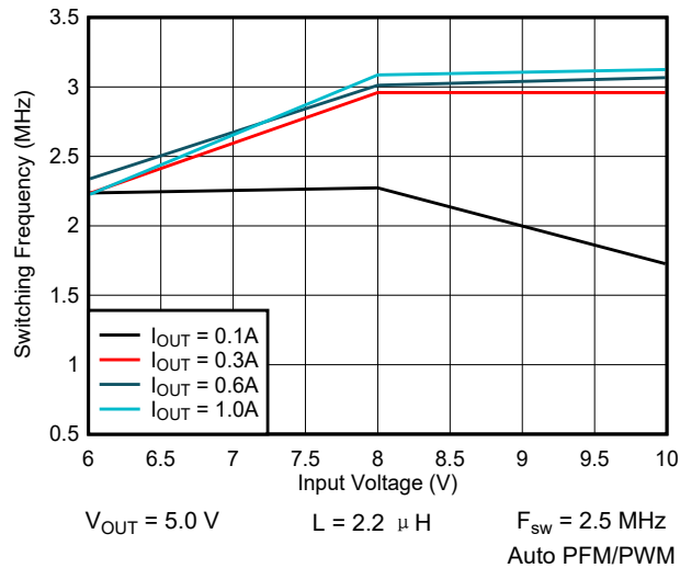
图 9-4. Switching Frequency vs Input Voltage
