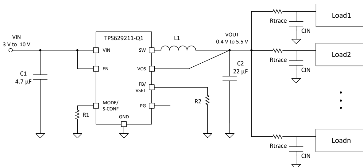
图 9-76. Multiple Loads Example
