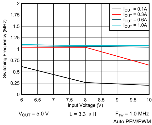
图 9-10. Switching Frequency vs Input Voltage
