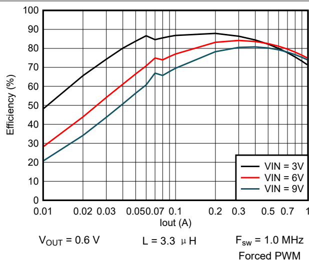
图 9-57. Efficiency vs Output Current
