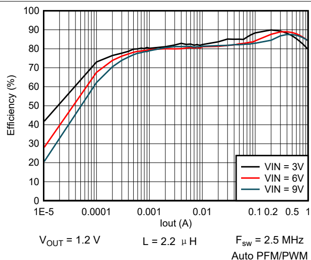
图 9-38. Efficiency vs Output Current
