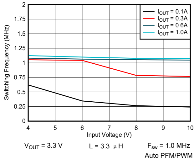
图 9-22. Switching Frequency vs Input Voltage
