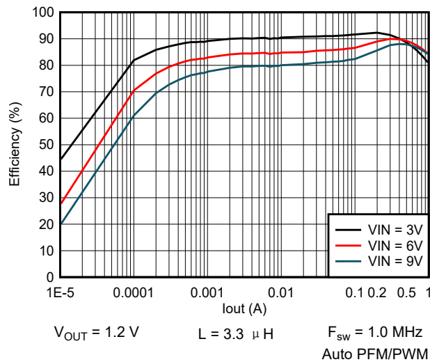
图 9-44. Efficiency vs Output Current
