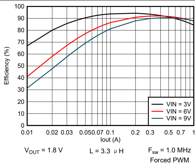
图 9-33. Efficiency vs Output Current
