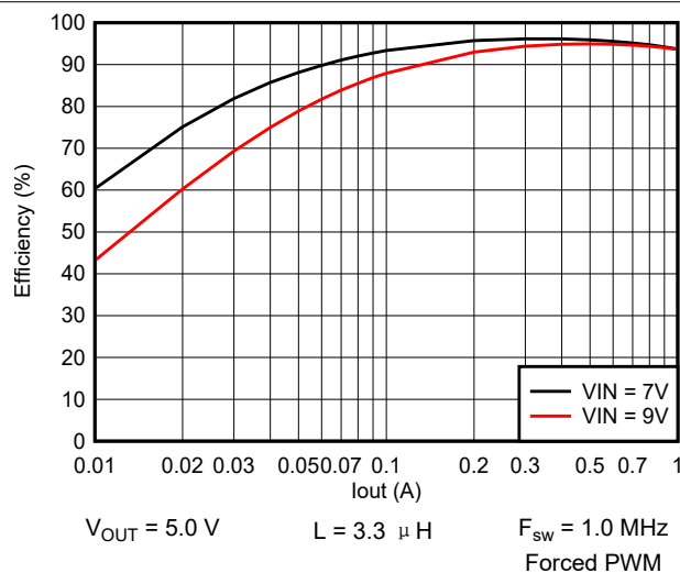
图 9-9. Efficiency vs Output Current
