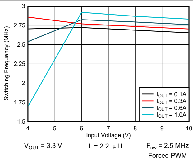
图 9-17. Switching Frequency vs Input Voltage
