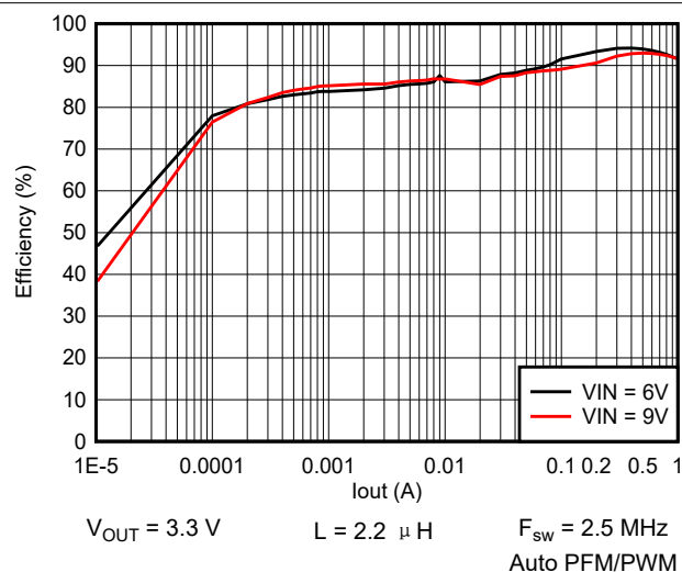
图 9-14. Efficiency vs Output Current
