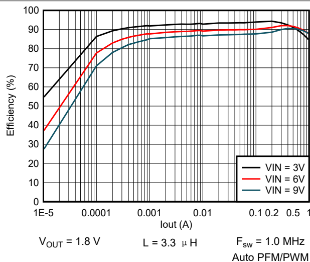
图 9-32. Efficiency vs Output Current
