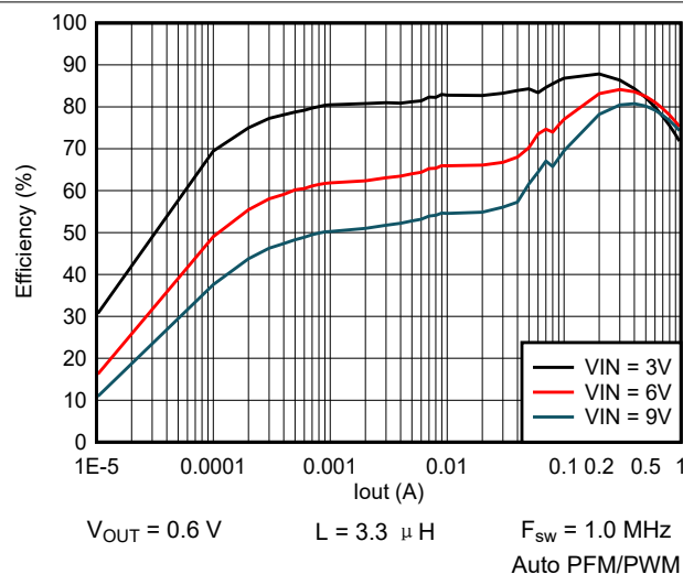
图 9-56. Efficiency vs Output Current
