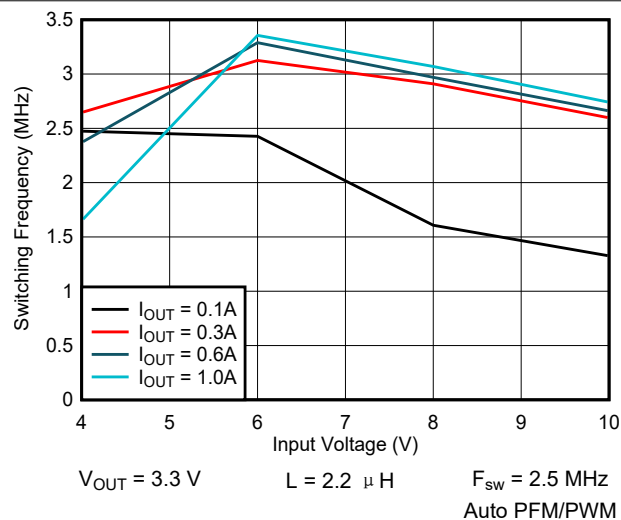
图 9-16. Switching Frequency vs Input Voltage
