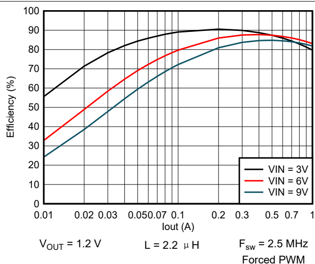
图 9-39. Efficiency vs Output Current
