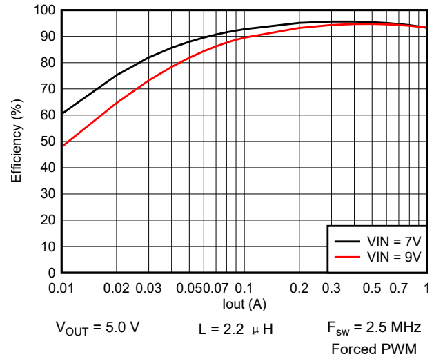
图 9-3. Efficiency vs Output Current
