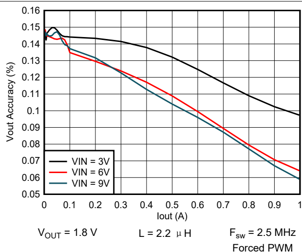
图 9-31. Output Voltage vs Output Current
