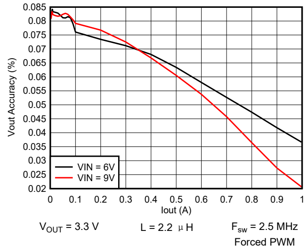
图 9-19. Output Voltage vs Output Current
