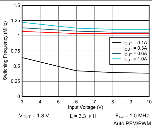
图 9-34. Switching Frequency vs Input Voltage
