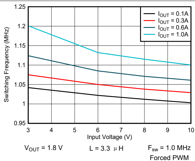
图 9-35. Switching Frequency vs Input Voltage
