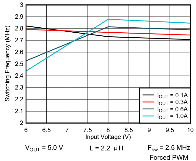
图 9-5. Switching Frequency vs Input Voltage
