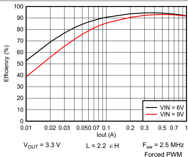
图 9-15. Efficiency vs Output Current
