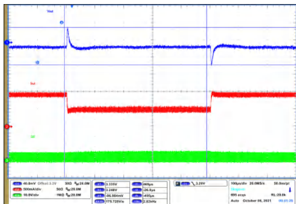
图 9-66. Shutdown Timing with Output Discharge Disabled
