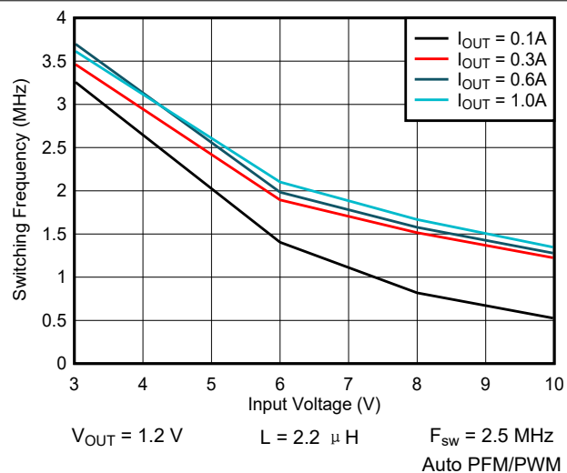
图 9-40. Switching Frequency vs Input Voltage
