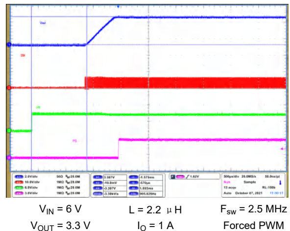
图 9-63. Start-Up Timing
