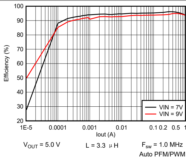
图 9-8. Efficiency vs Output Current
