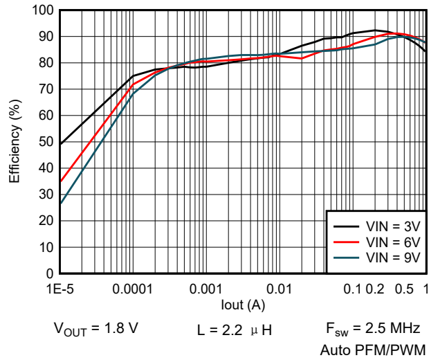
图 9-26. Efficiency vs Output Current
