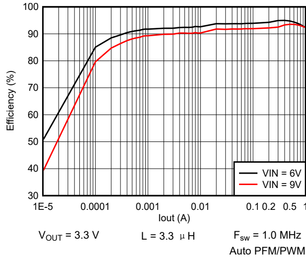
图 9-20. Efficiency vs Output Current
