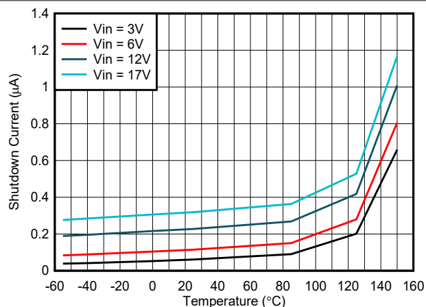
图 7-2. Typical Shutdown Current vs Temperature
