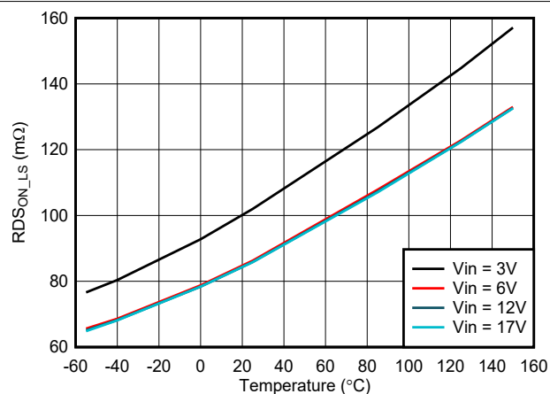
图 7-12. Low-Side R_{DS(ON)} vs Temperature
