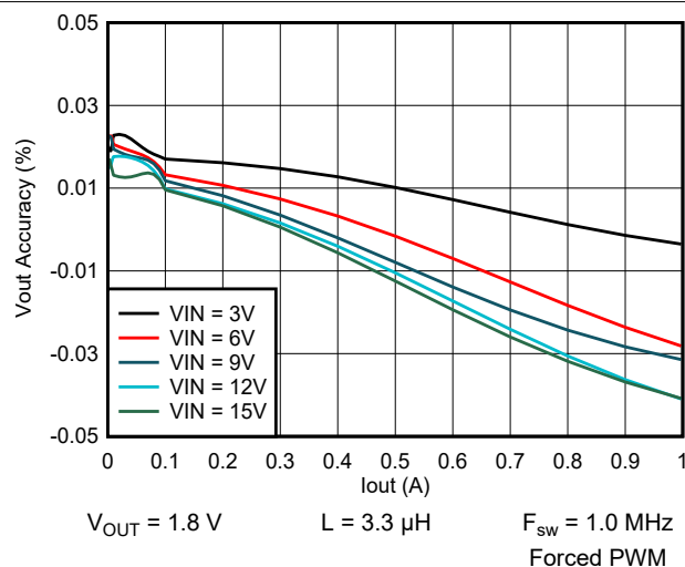
图 9-37. Output Voltage vs Output Current
