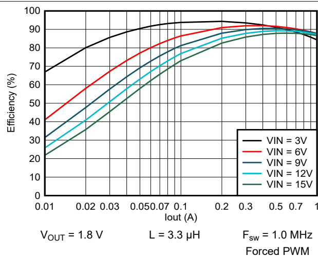
图 9-33. Efficiency vs Output Current
