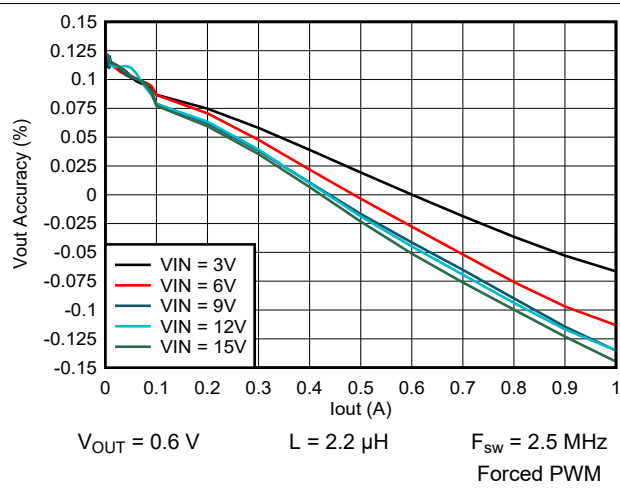
图 9-55. Output Voltage vs Output Current
