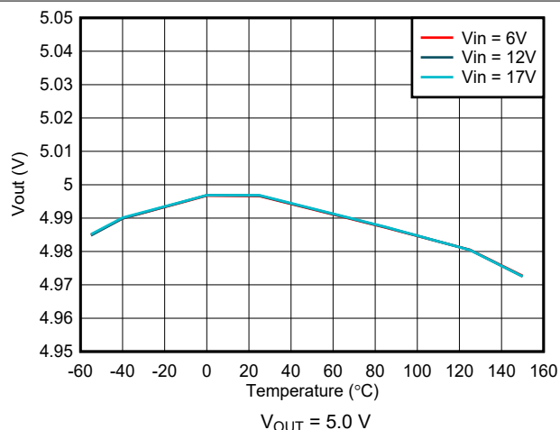
图 7-4. Output Voltage Accuracy – VSET Selected
