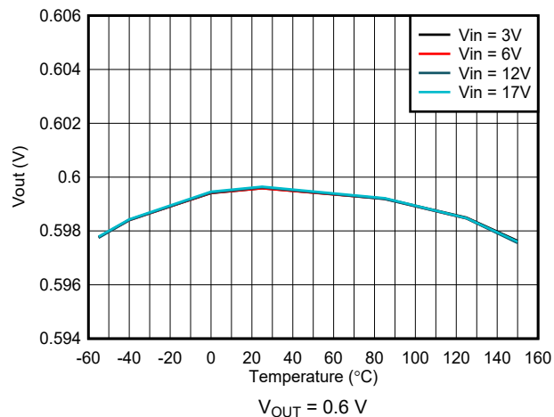
图 7-8. Output Voltage Accuracy – VSET Selected
