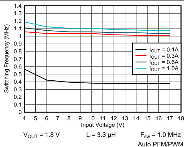
Figure 9-34. Switching Frequency vs Input Voltage
