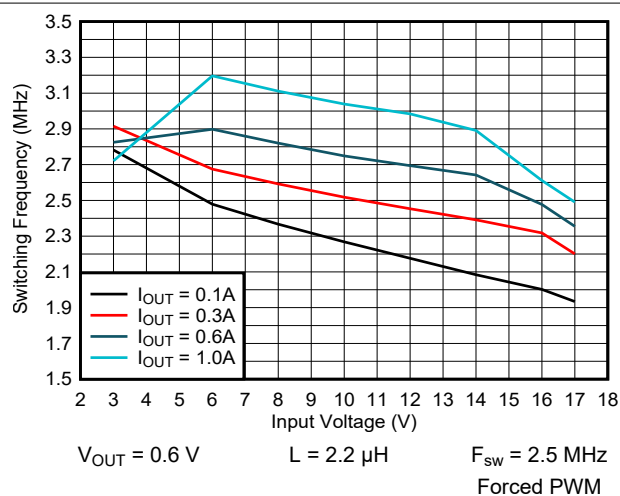
图 9-53. Switching Frequency vs Input Voltage
