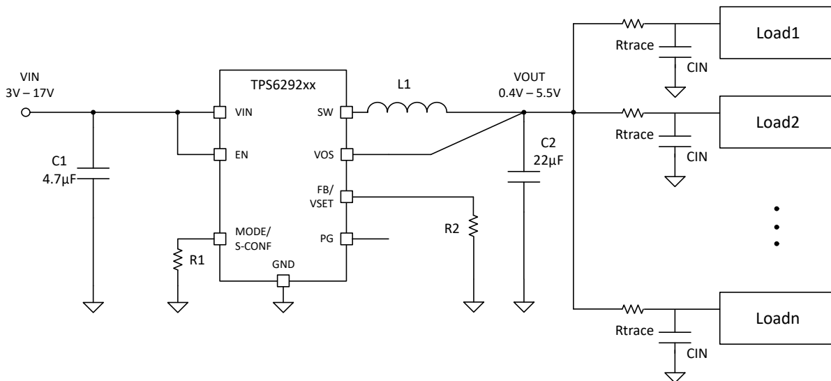
图 9-83. Multiple Loads Example
