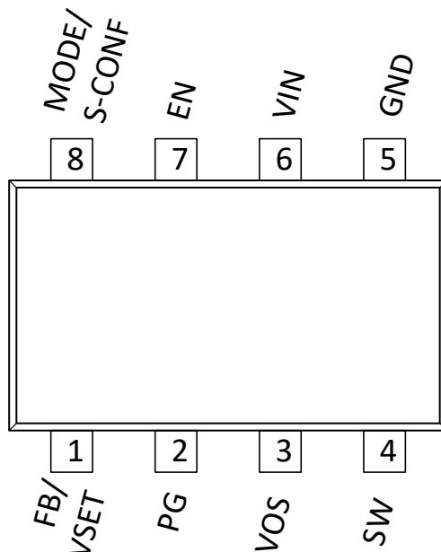
图 6-1. TPS629210E 8-Pin DRL SOT-5X3 Pinout
