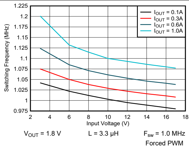
图 9-35. Switching Frequency vs Input Voltage
