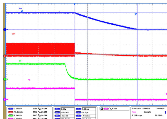
图 9-69. Shutdown Timing with Output Discharge Disabled
