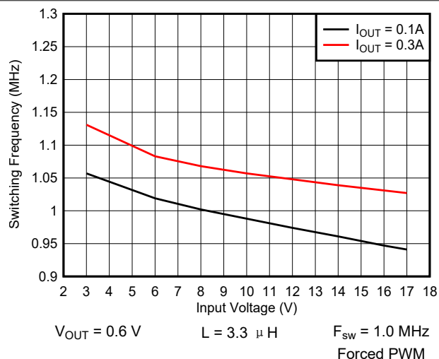
图 9-59. Switching Frequency vs Input Voltage
