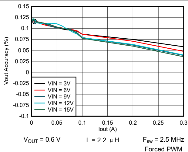
图 9-55. Output Voltage vs Output Current
