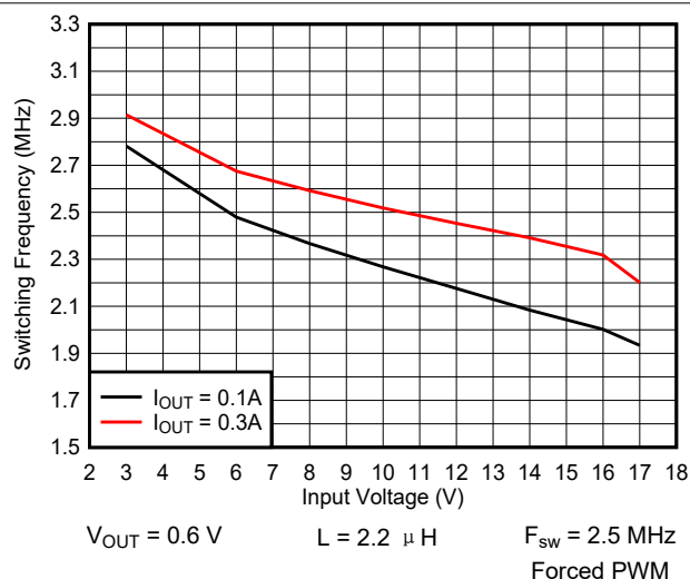
图 9-53. Switching Frequency vs Input Voltage
