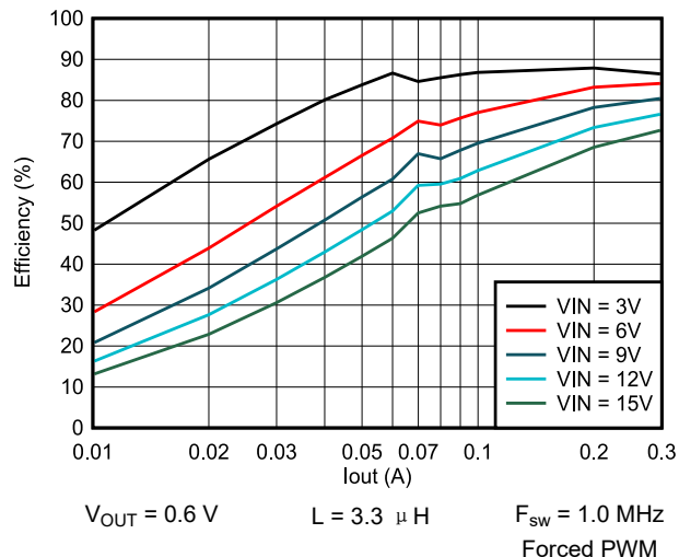
图 9-57. Efficiency vs Output Current
