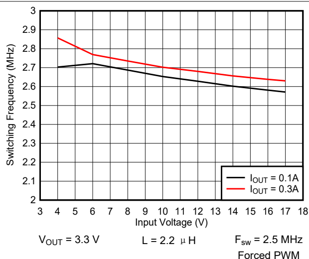
图 9-17. Switching Frequency vs Input Voltage
