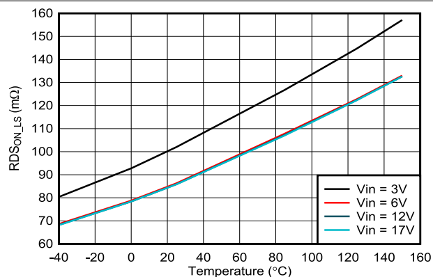
图 7-12. Low-Side R_{DS(on)} vs Temperature
