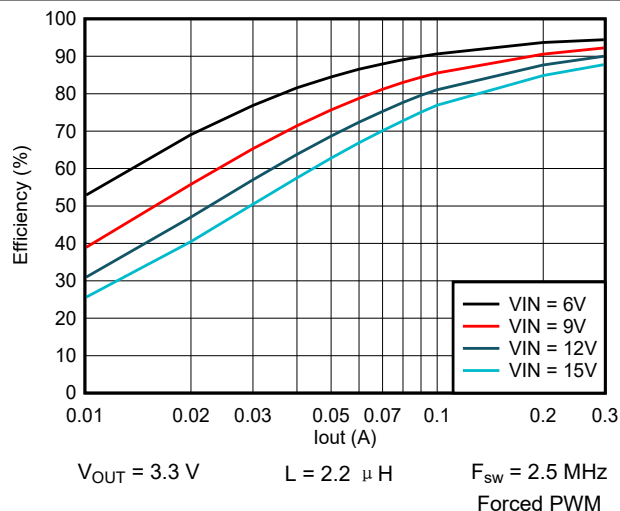
图 9-15. Efficiency vs Output Current
