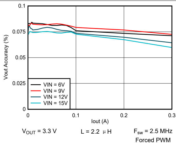
图 9-19. Output Voltage vs Output Current
