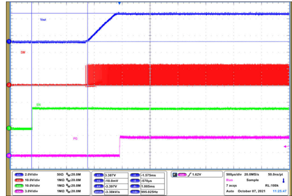
图 9-63. Start-Up Timing
