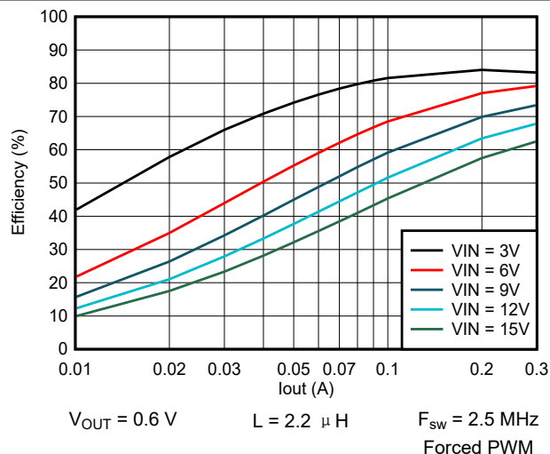
图 9-51. Efficiency vs Output Current
