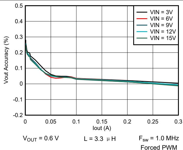
图 9-61. Output Voltage vs Output Current
