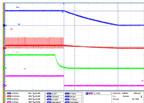
图 9-65. Shutdown Timing with Output Discharge Enabled
