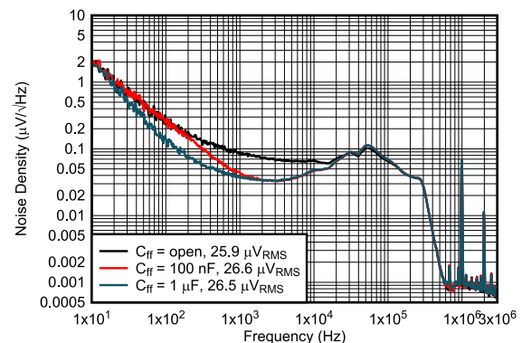
图 6-34. Output Noise Density vs Frequency
