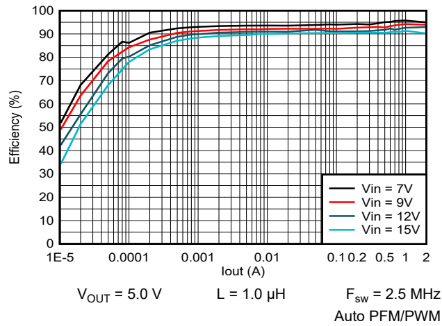
图 9-40. Efficiency vs Output Current
