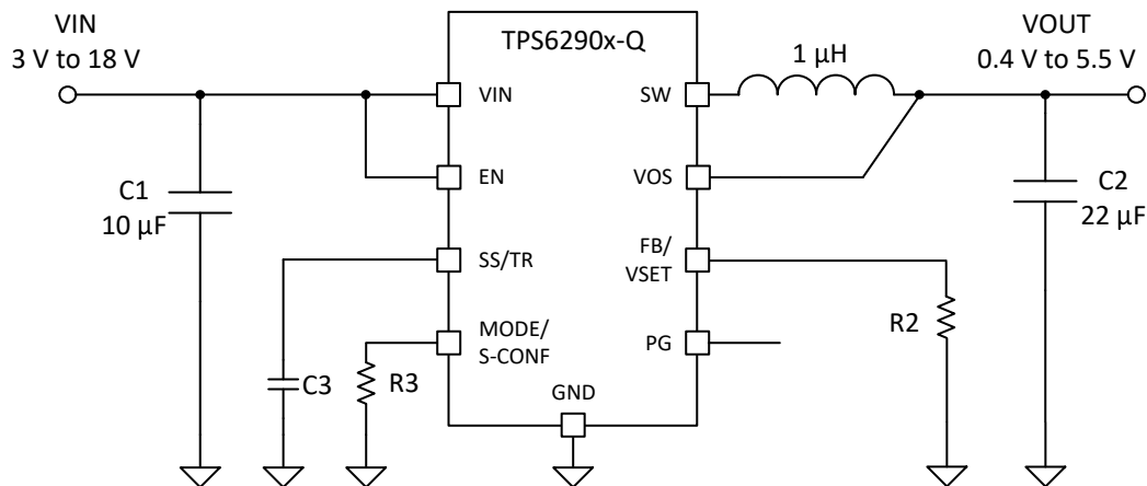
图 9-39. Typical Application Circuit (VSET)
