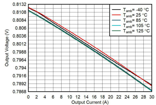
V_{IN} = 3.3V FPWM ; TPS6287B25 压 降启用 V_{OUT} = 0.8V
