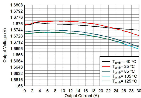
V_{IN} = 3.3V FPWM ; TPS6287B25 V_{OUT} = 1.675V 压降禁用
