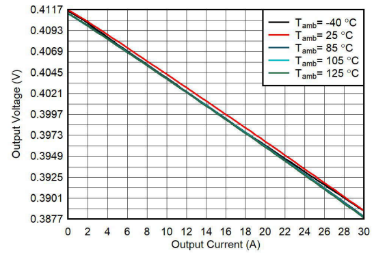
V_{IN} = 3.3V FPWM ; TPS6287B25 压 降启用 V_{OUT} = 0.4V
