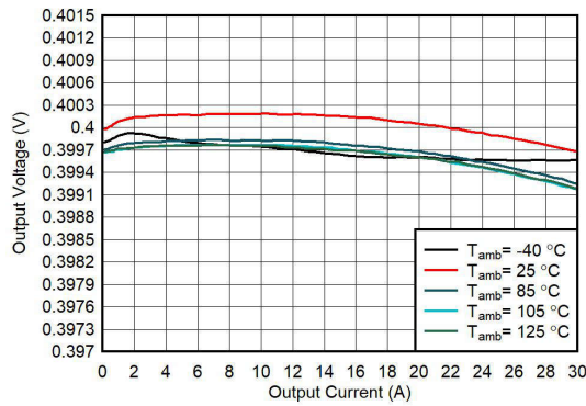
V_{IN} = 3.3V FPWM ; TPS6287B25 V_{OUT} = 0.4V 压降禁用
