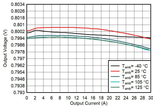
V_{IN} = 3.3V FPWM ; TPS6287B25 V_{OUT} = 0.8V 压降禁用
