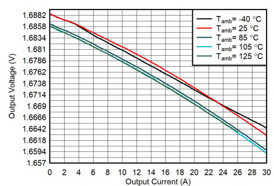
V_{IN} = 3.3V FPWM ; TPS6287B25 压 降启用 V_{OUT} = 1.675V
