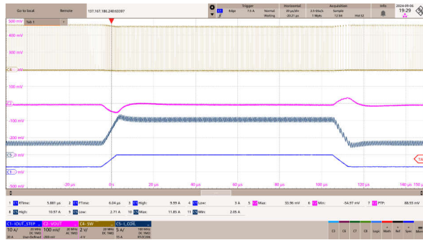
V_{IN} = 5.0V TPS6286A10 BOM = 4 \times 22 \mu F V_{OUT} = 0.9V I_{OUT} = 4A \text{ 至 } 10A, 1A/\mu s
